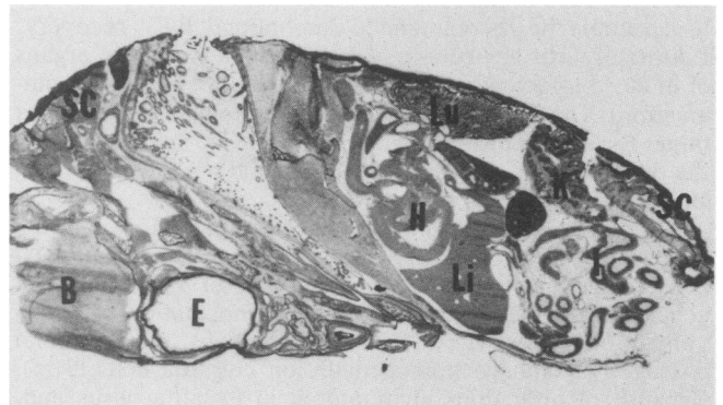
FIG. 1. Hematoxylin-and-eosin-stained longitudinal section of a 15-day-old chicken embryo. Individual organs: B, brain; E, eye; H, heart; Li, liver; Lu, lung; I, intestine; S, spleen; SC, spinal cord; K, kidney.
