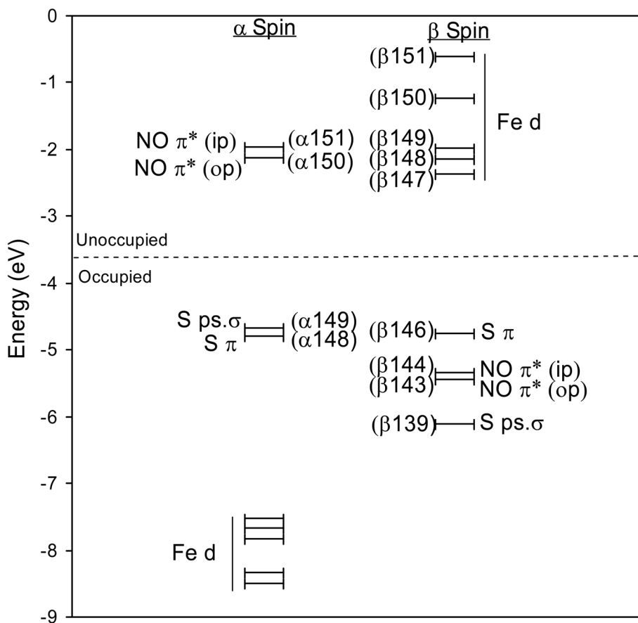
Figure 6. Molecular orbital diagram of Fe-IPNS-ACV-NO. The 5 lowest unoccupied \beta orbitals are comprised of mostly Fe d character, while the 2 lowest unoccupied \alpha orbitals are comprised of mostly NO \pi^* character, consistent with an electronic structure description of a high-spin Fe III antiferromagnetically coupled to NO - .
