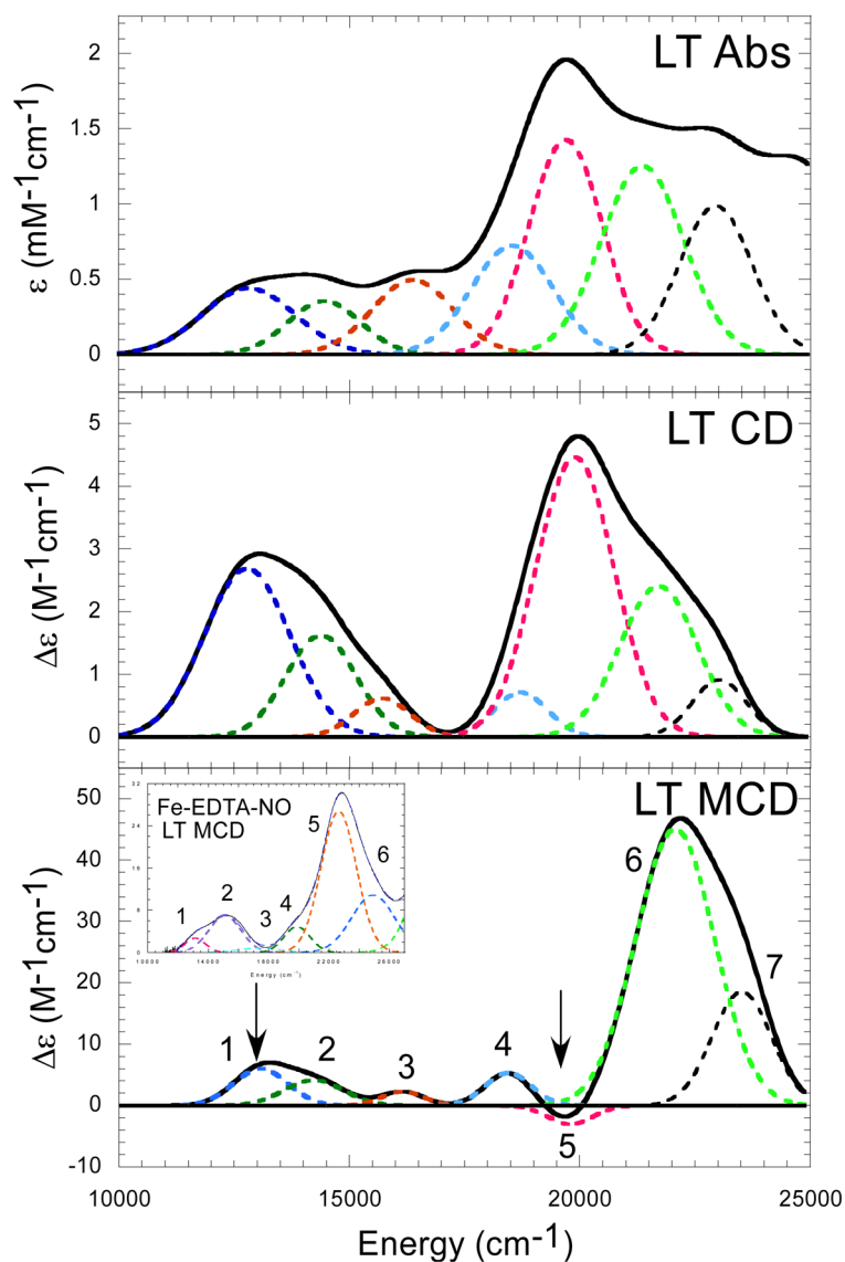
Figure 2. Absorbance (10K, top), CD (5K, middle) and MCD (5K,7T, bottom) spectra collected for Fe-IPNS-ACV-NO with Gaussian best fits. Comparison to the MCD spectrum of Fe-EDTA-NO (inset) reveals two new spectral features seen in the spectra upon addition of ACV to Fe-IPNS-NO (arrows).
