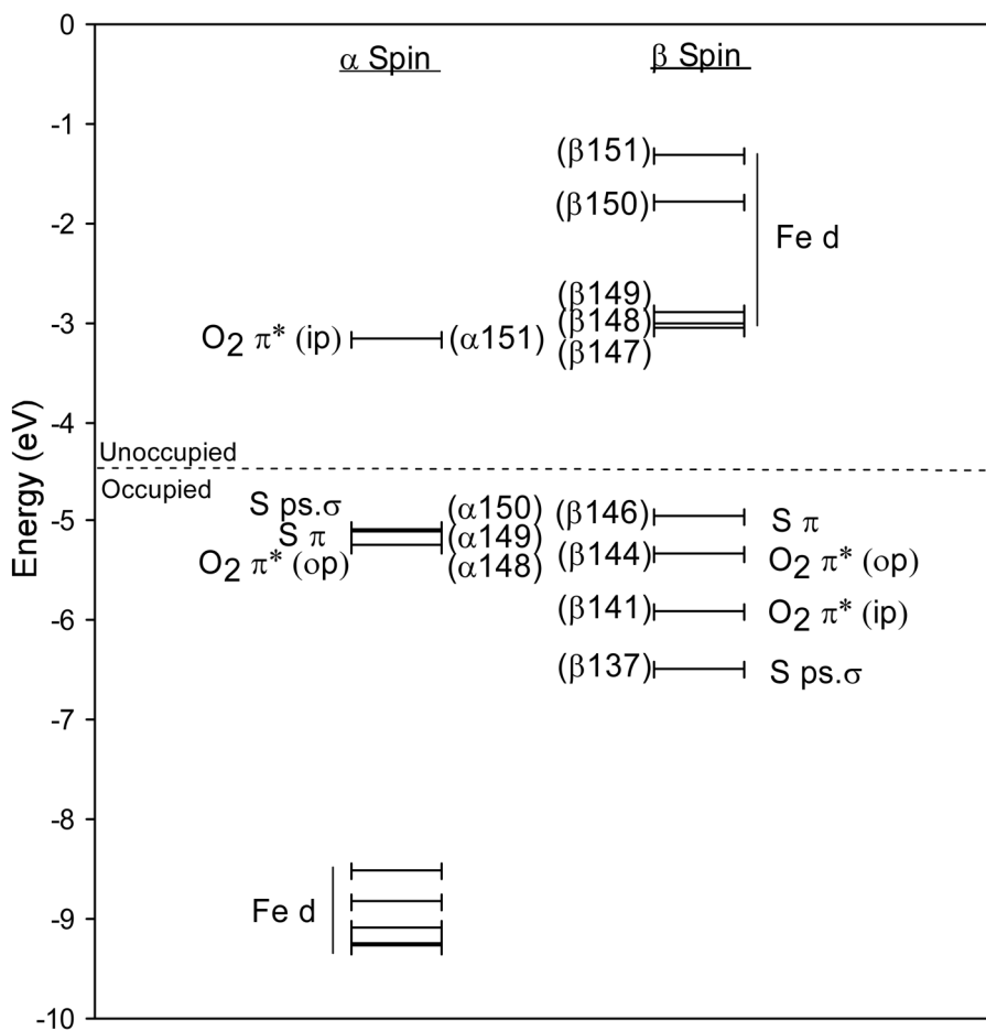
Figure 9. Molecular orbital diagram of Fe-IPNS-ACV-O 2 . The 5 lowest unoccupied \beta orbitals are comprised of mostly Fe d character, while the lowest unoccupied \alpha orbital is comprised of mostly O 2 \pi^* character, consistent with an electronic structure description of a high-spin Fe III antiferromagnetically coupled to O 2 - .
