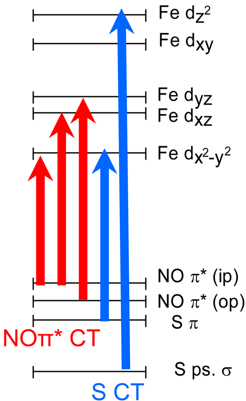
Figure 7. \Delta SCF charge transfer transition for the Fe-IPNS-ACV-NO complex calculated using ADF/BP86/TZV with Z_{\text{eff}} = 25.6 .
