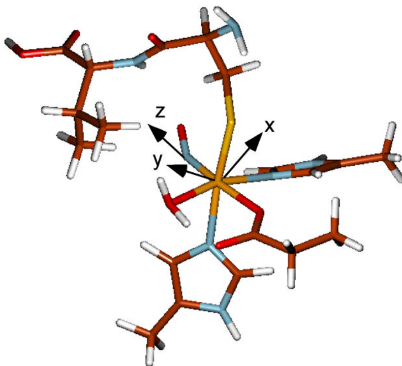
Figure 4. UBP86+10%HF/6-311G*/6-31G* Optimized Fe-IPNS-ACV-NO complex.
