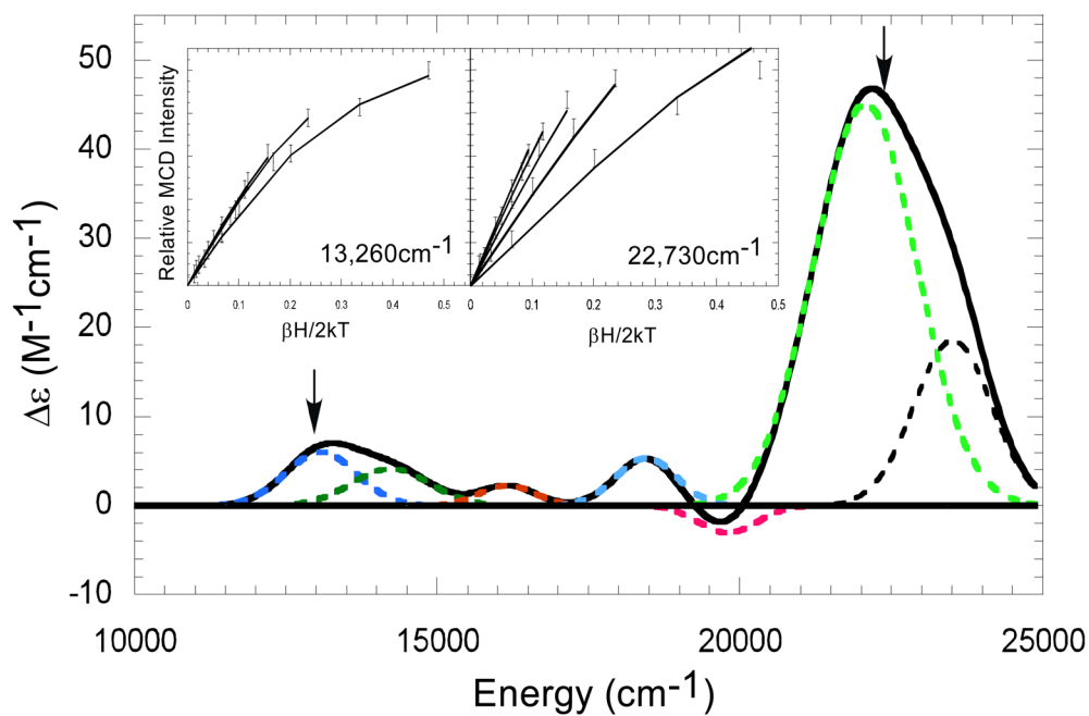
Figure 3. Fe-IPNS-ACV-NO VTVH MCD data collected at 13,260 \text{cm}^{-1} (left) and 22,730 \text{cm}^{-1} (right) demonstrate different nesting behaviors. (Arrows indicate energy where the isotherms were collected.)
