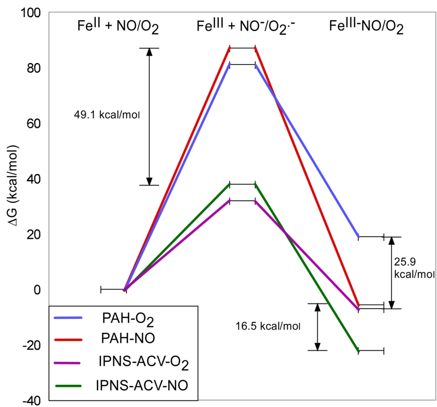
Figure 10. Energy profiles of NO/O 2 binding to Fe-IPNS-ACV and Fe-PAH.
