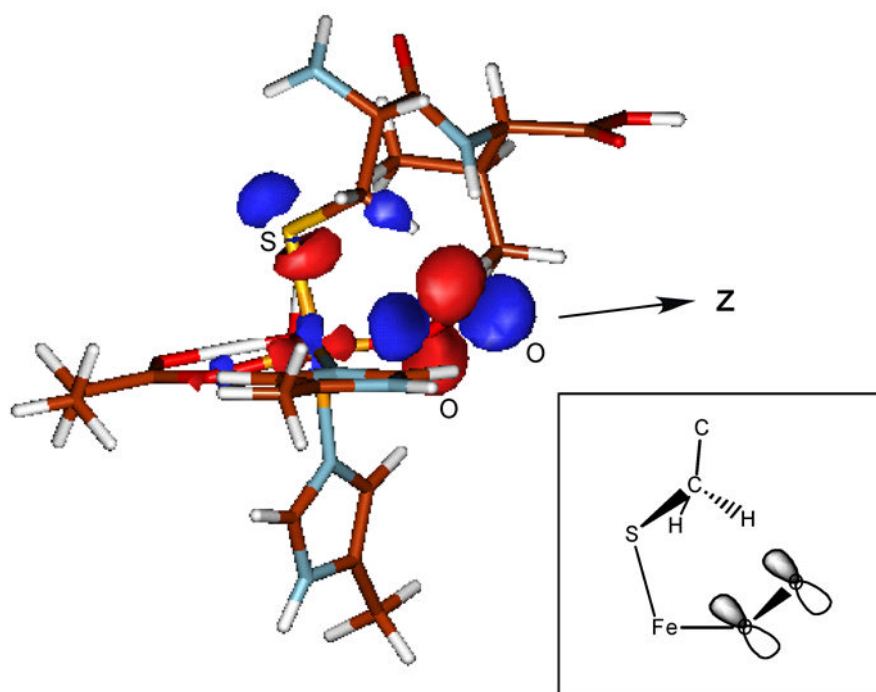
Figure 11. Fe-IPNS-ACV-O 2 FMO with proper orientation for H-atom abstraction of cysteine β-methylene H from ACV.
