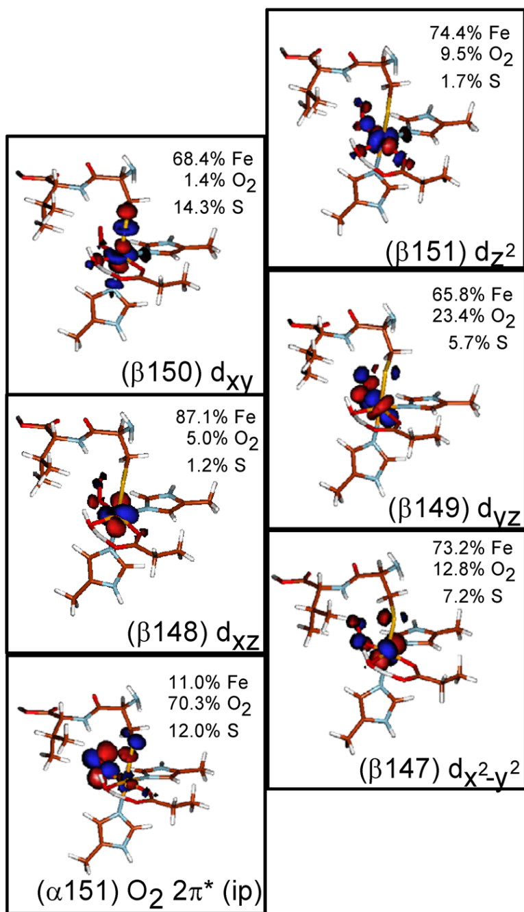
Figure 8. Contours of the lowest unoccupied \alpha and \beta molecular orbitals from the ground state wavefunction of Fe-IPNS-ACV-O 2
