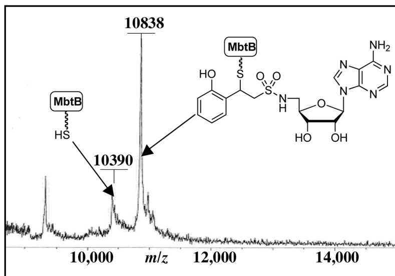
Figure 2. MALDI-TOF of the ArCP domain of MbtB modified with affinity probe 1 . MS: calcd for [C7S holo-ArCP] 10376; calcd for [C7S holo-ArCP+ 1 ] 10843.
