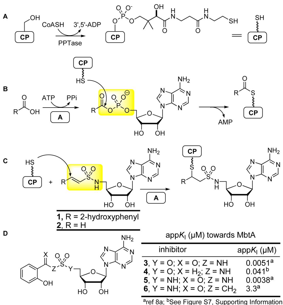
Figure 1. Carrier Protein (CP) Modifications. (A) The Ppant prosthetic group on an invariant serine residue is installed post-translationally by a PPTase. (B) Loading of CPs mediated by adenylation domains. (C) A mechanism-based CP affinity probe for CP domains incorporates a Michael acceptor. (D) Reversible bisubstrate inhibitors of MbtA. 8
