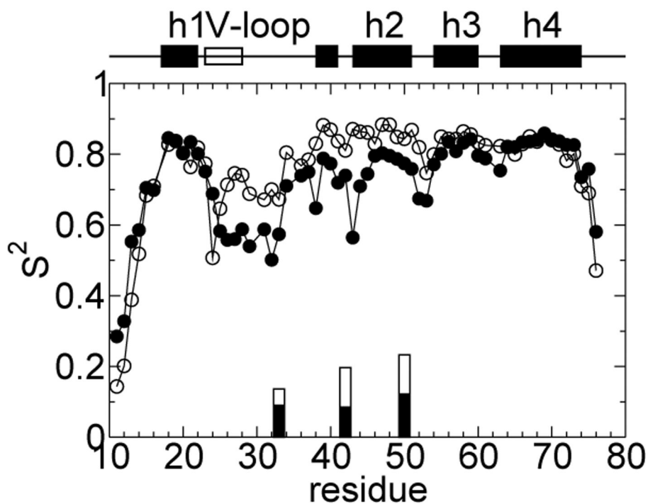
Figure 3. Computed NMR order parameters ( S^2 ) are plotted against amino acid sequence for state 1 (open) and 2 (filled symbols). The back-bone N-H order parameters are represented as circles while the methyl C-H parameters are represented as bars. For the latter, only those within the N-terminal and interface hydrophobic clusters displaying significant changes ( > 25\% ) are shown.
