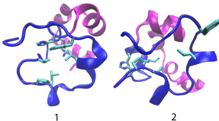
Figure 1. Representative conformations for state 1 and 2 obtained as centroids of the largest conformational cluster from the REX-CPHMD simulations at pH 7. The N- and C-terminal subdomains are colored blue and magenta, respectively. The side chains of the N-terminal hydrophobic cluster are shown in liquorice.
