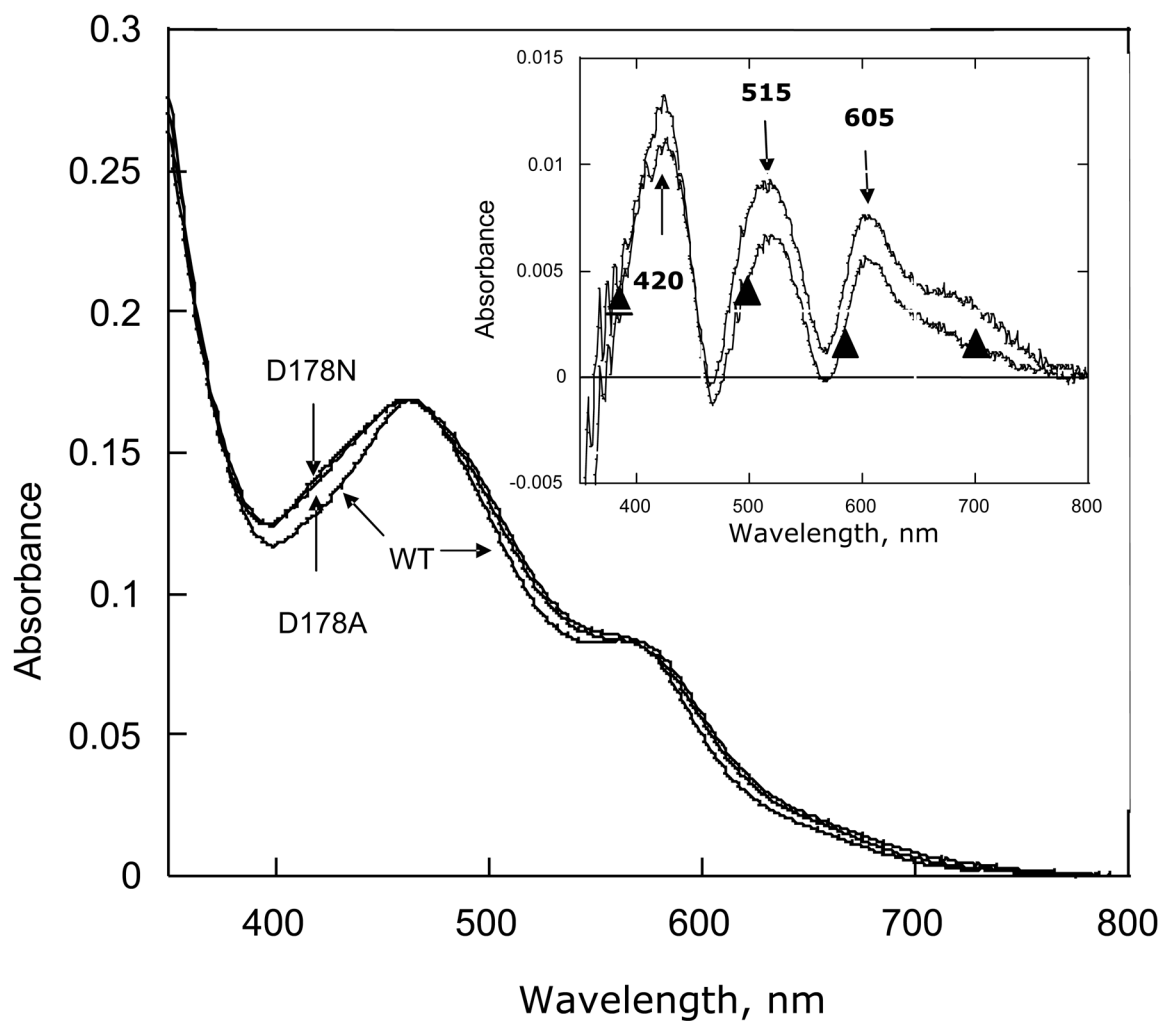
Figure 2. Absorbance spectra of recombinant PDO (35 μM) in 0.1 M HEPES pH 7.5, 3 mM phthalate. WT PDO, PDO D178N and PDO D178A. Insert: Difference spectra of PDO D178N (▲) and PDO D178A spectra minus the WT PDO-Fe(II) spectrum.
