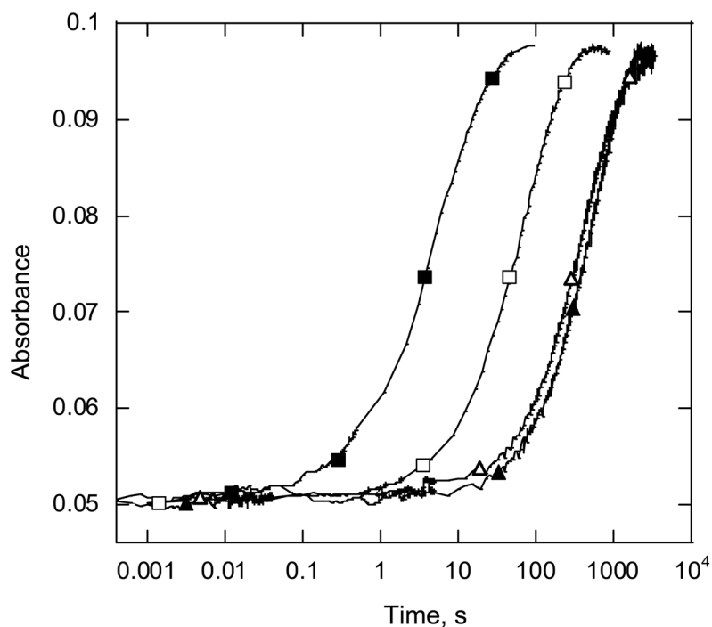
Figure 8. Oxidation of reduced D178N-APO PDO by oxygen. D178N-APO (20 \mu\text{M} ) was mixed with 125 \mu\text{M} \text{O}_2 in 0.1M HEPES pH 7.8.0 at 22 ^\circ\text{C} (▲), in the presence of 3 mM phthalate in the oxygenated buffer (△), preincubated with 500 \mu\text{M} FAS (□) and in the presence of 3 mM phthalate, as well as preincubating with 500 \mu\text{M} FAS (■). Data for D178A are similar (not shown). All concentrations (except for the FAS) are those after mixing in the stopped-flow spectrophotometer. Traces were recorded at 575 nm.
