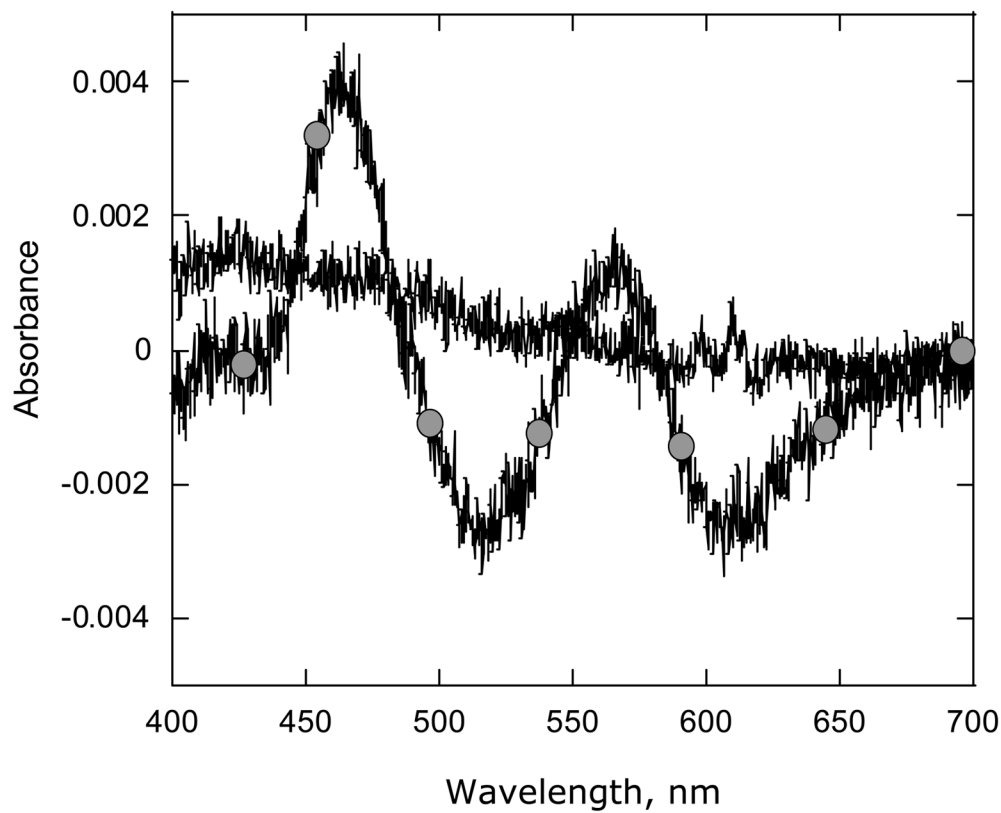
Figure 7. Effect of phthalate binding on the absorbance spectrum of PDO WT-APO (●) and of the D178N PDO variant (–). PDO (78 \mu M) in phthalate free buffer (0.1 M HEPES, pH 7.8) was mixed with an equal volume of buffer containing 10 mM phthalate. Presented are the difference spectra (with phthalate minus no phthalate).
