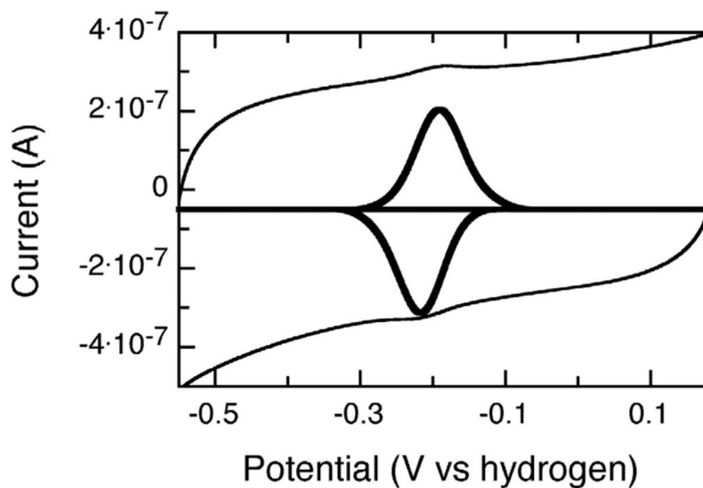
Figure 4. PFV response of D178N mutant of PDO adsorbed upon a graphite electrode, baseline subtracted data are inset into the voltammogram, and shown in bold. Conditions as described in Materials and Methods.
