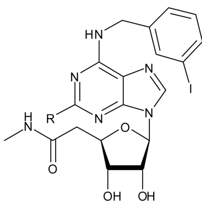
R = H: IB-MECA R = Cl: 2-Cl-IB-MECA
