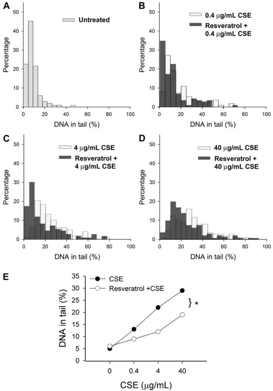
Fig. 9. Results from comet assay experiments. CAECs were treated with Res ( 10^{-5} mol/l for 24 h) followed by exposure to CSE (from 0.4 to 40 µg/ml). A–D : frequency distribution of tail DNA content in untreated control cells ( A ) and CAECs treated with CSE or Res plus CSE [ B–D ; damaged DNA migrates during electrophoresis from the nucleus toward the anode, forming a shape of a comet with a head (cell nucleus with intact DNA) and a tail (relaxed and broken DNA)]. E : summary data. Res pretreatment significantly attenuated CSE-induced increases in tail DNA content. * P < 0.05 .
