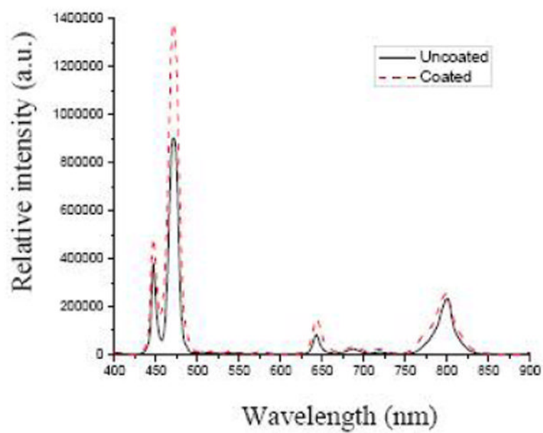
Figure 2. Photoluminescence spectra of NaYF 4 :Yb 3+ ,Tm 3+ nanoparticles before and after being coated with Ru(bpy) 3 2+ -doped silica.
