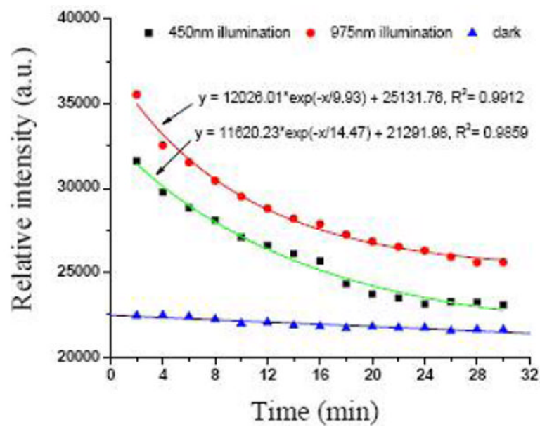
Figure 4. Change of intensity of ADPA emission at 420 nm, excited at 378 nm, for the respective solutions. The lines represent the fitting of the data points.
