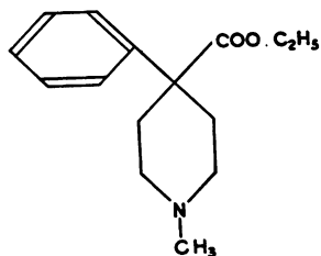
pethidine
