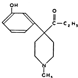
1-methyl-4-(4-hydroxyphenyl)-4-propionyl-piperidine
