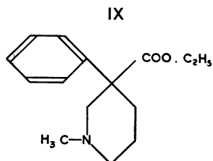
1-methyl-3-phenyl-piperidine-3-carboxylic acid ethyl ester, \beta -pethidine, iso -pethidine, iso -dolantin
