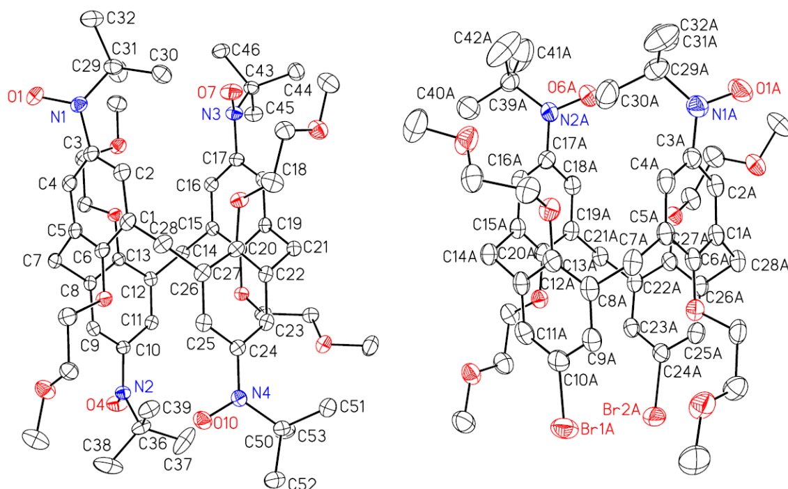
Figure 3. Molecular structure and conformation for nitroxide tetradiradical 1 (left) and diradical 2 (right) with constrained conformations of 1,3-alternate calix[4]arene. Carbon, nitrogen, and oxygen atoms are depicted with thermal ellipsoids set at the 50% probability level. Only one of the two unique molecules of 2 and without the solvent of crystallization (benzene) is shown.
