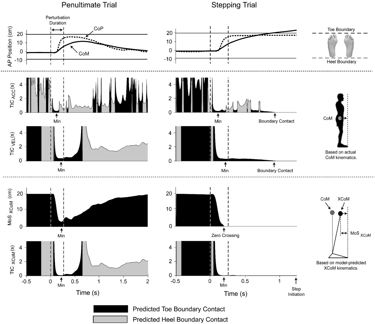
Figure 3. Example of perturbation response for penultimate and stepping trials. Top graphs show center of mass (CoM) and center of pressure (CoP) kinematics, and toe and heel positions. Middle graphs show CoM time-to-contact (TiC) computed by including (TiC ACC ) and not including (TiC VEL ) acceleration information. Bottom graphs show the margin of stability (MoS XCoM ) and TiC (TiC XCoM ) of the extrapolated center of mass (XCoM) based on an inverted pendulum model (Hof et al. 2005).
