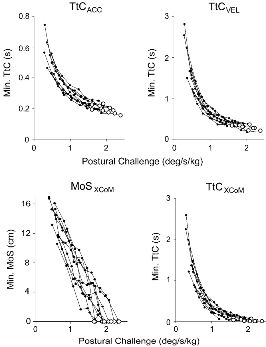
Figure 4. Top: Minimum time-to-contact (TtC) based on the kinematics of the center of mass (CoM), computed with and without acceleration information (TtC ACC and TtC VEL , respectively), as a function of postural challenge level for all subjects. Bottom: Minimum margin of stability (MoS XCoM ) and TtC (TtC XCoM ) of the extrapolated center of mass, which are based on an inverted pendulum model. Enlarged open circles indicate stepping trials. Note that TtC ACC vertical scaling is different from TtC VEL and TtC XCoM .
