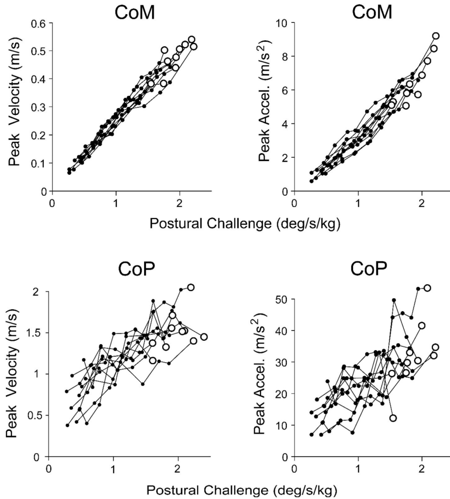
Figure 2. Relationship between postural challenge and peak forward center of mass (CoM) velocity and acceleration (top), and peak forward center of pressure (CoP) velocity and acceleration (bottom). Each line represents data from one subject. Enlarged open circles represent stepping trials.
