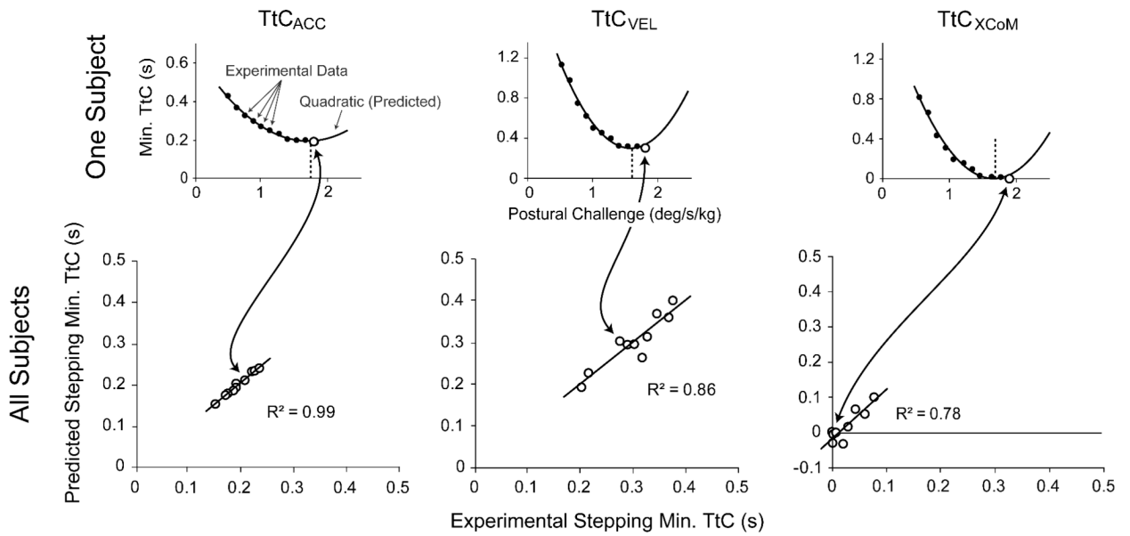
Figure 5. Top Row: Experimental minimum time-to-contact (TtC) data and fitted quadratics for one subject when acceleration information is included (TtC ACC , left), and not included (TtC VEL , middle). The TtC of a model extrapolated center of mass (XCoM) is also shown (TtC XCoM , right). Closed and open circles indicate non-stepping and stepping trials, respectively. Bottom Row: Linear correlations between the experimental and predicted (vertices of quadratic functions) minimum TtC values for stepping responses of all subjects using the different TtC calculation methods.
