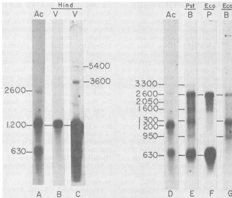
FIG. 4. RNA blot analysis of AcMNPV RNA. Poly(A) + RNA was isolated from the cytoplasm of AcMNPV-infected cells at 48 h p.i. and denatured with formaldehyde. Samples of 2 \mu g were electrophoresed in a 1% agarose–2.2 M formaldehyde gel, transferred to nitrocellulose, and hybridized to 32 P-labeled AcMNPV (lanes A and D) or cloned DNA fragments Hind III-V (lanes B and C), Pst I-B (lane E), Eco RI-P (lane F), and Eco RI-B (lane G). Lanes A, B, D, E, F, and G were exposed for 6 h, and lane C was exposed for 48 h at –80°C with the aid of an intensifying screen. The sizes of AcMNPV RNAs are given in nucleotides and were determined relative to E. coli 5S, 16S, and 23S ribosomal RNA standards.
