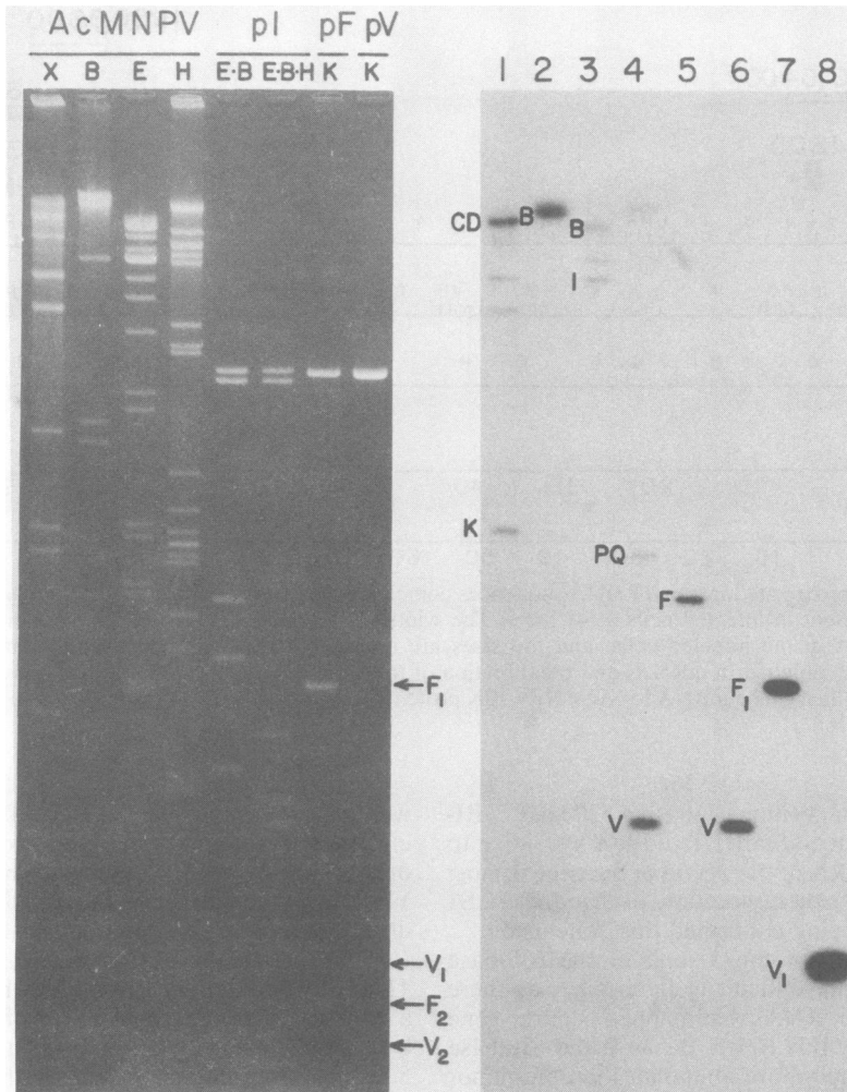
FIG. 6. Hybridization analysis of AcMNPV cDNA. A ^{32}\text{P} -labeled cDNA probe was made by primed synthesis with avian myeloblastosis virus reverse transcriptase, using the 3' ends of AcMNPV poly(A) + RNA isolated from infected cells at 48 h p.i. as a template. The cDNA probe was hybridized to AcMNPV DNA (right panel) restricted with Xho I (X), Bam HI (B), Eco RI (E), and Hind III (H) and to cloned plasmids Eco RI-I (pI) restricted with Eco RI and Bam HI (E · B) or Eco RI, Bam HI, and Hind III (E · B · H); cloned Bam HI-F (pF) restricted with Bam HI and Kpn I (K); and cloned Hind III-V (pV) restricted with Hind III and Kpn I (K) (lanes 1 through 8, respectively). Kpn I subfragments of AcMNPV Bam HI-F ( F_1 and F_2 ) and Hind III-V ( V_1 and V_2 ) are marked. An ethidium bromide-stained gel of these fragments is shown in the left panel. Certain fragments discussed in the text are labeled.
