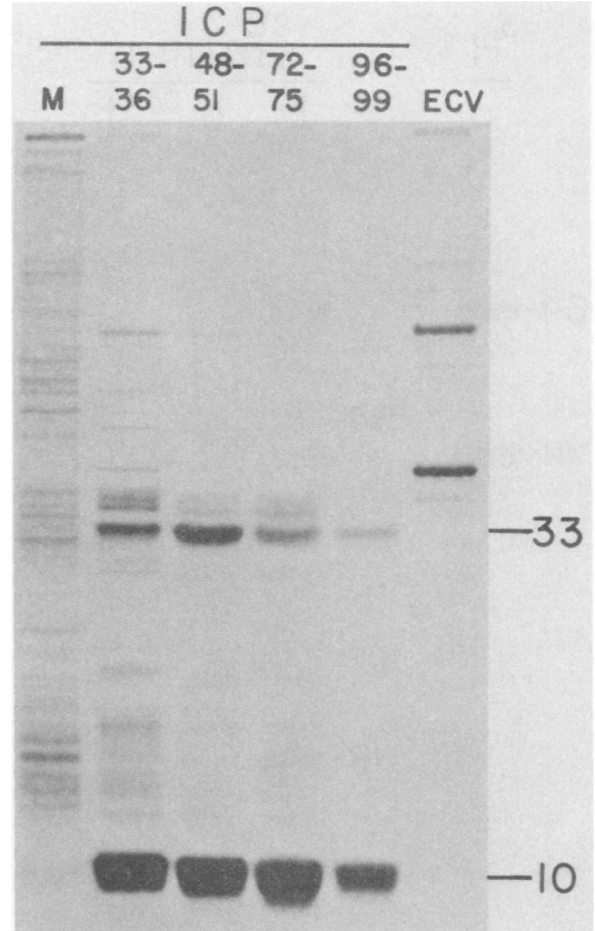
FIG. 1. Pulse-labeled AcMNPV-infected cell proteins. S. frugiperda cells were infected with AcMNPV and labeled with L- ^3 H]leucine at 33 to 36, 48 to 51, 72 to 75, and 96 to 99 h p.i. Mock-infected cell proteins (M) were labeled at 33 to 36 h, and L- ^3 H]leucine-labeled AcMNPV extracellular virus (ECV) was purified from infected cells labeled at 0 to 48 h p.i. Labeled proteins were electrophoresed in 10% polyacrylamide, prepared for fluorography, and exposed for 4 days at -80^{\circ}\text{C} . The 33K and 10K polyhedrin and 10K protein are indicated by 33 and 10, respectively.
