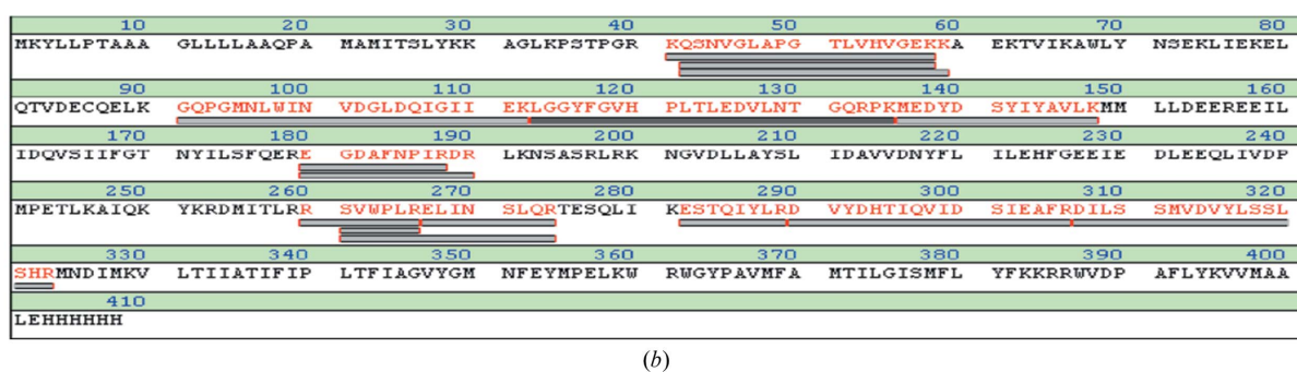
Figure 2 CorA purification. (a) Coomassie-stained SDS-PAGE of purified M. mazei CorA. Lane MW, molecular-weight markers (170, 130, 100, 70, 55, 40, 35, 25, 15 and 10 kDa); lane CorA, two-step purified M. mazei CorA. (b) Peptide mass-fingerprint MALDI-TOF identification using the sequence of M. mazei CorA and the band shown in Fig. 2(a). The sequence coverage was 35.5%. Grey bars indicate matching peptides.
