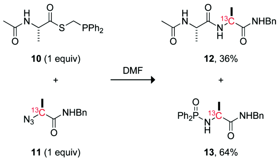
SCHEME 2. Reaction of Alanyl Phosphinothioester 10 with Alanyl Azide 11
