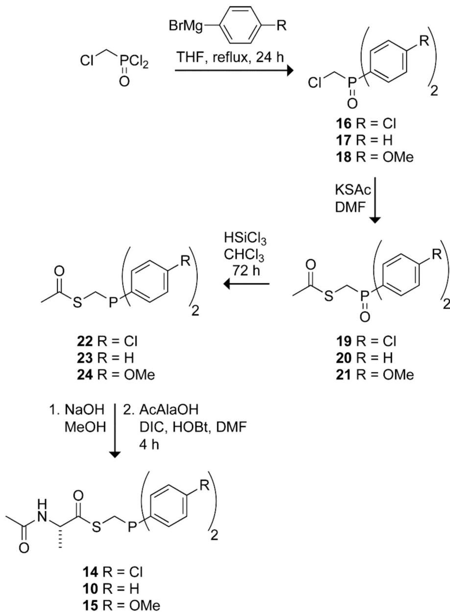
SCHEME 3. Synthesis of Alanyl Phosphinothioesters 10, 14, and 15
