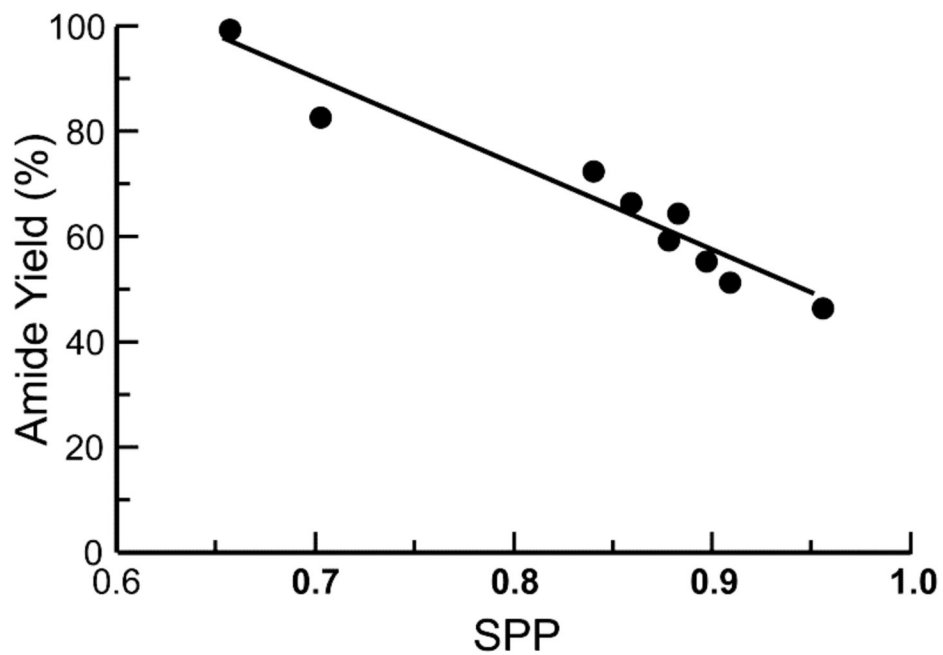
FIGURE 2. Plot of the yield of amide 12 product versus SPP value for the reaction of alanyl phosphinothioester 15 with ^{13}\text{C} -labeled alanyl azide 11 . The lines depict a linear least-squares fit of the data.
