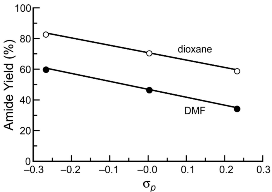
FIGURE 1. Plot of the yield of amide 12 product versus Hammett \sigma_p value for the reaction of alanyl phosphinothioesters 10 , 14 , and 15 with ^{13}\text{C} -labeled alanyl azide 11 in DMF and dioxane. The lines depict a linear least-squares fit of the data.
