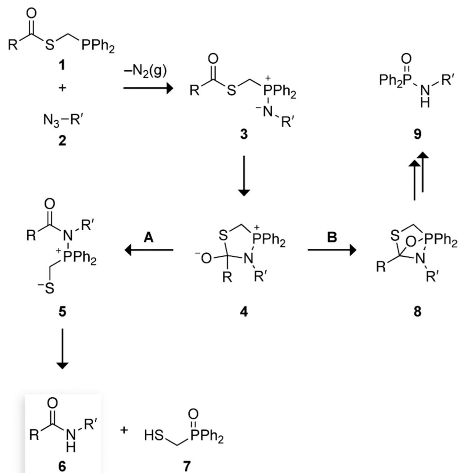
SCHEME 1. Putative Mechanism for the Traceless Staudinger Ligation Mediated by (Diphenylphosphino) methanethiol
