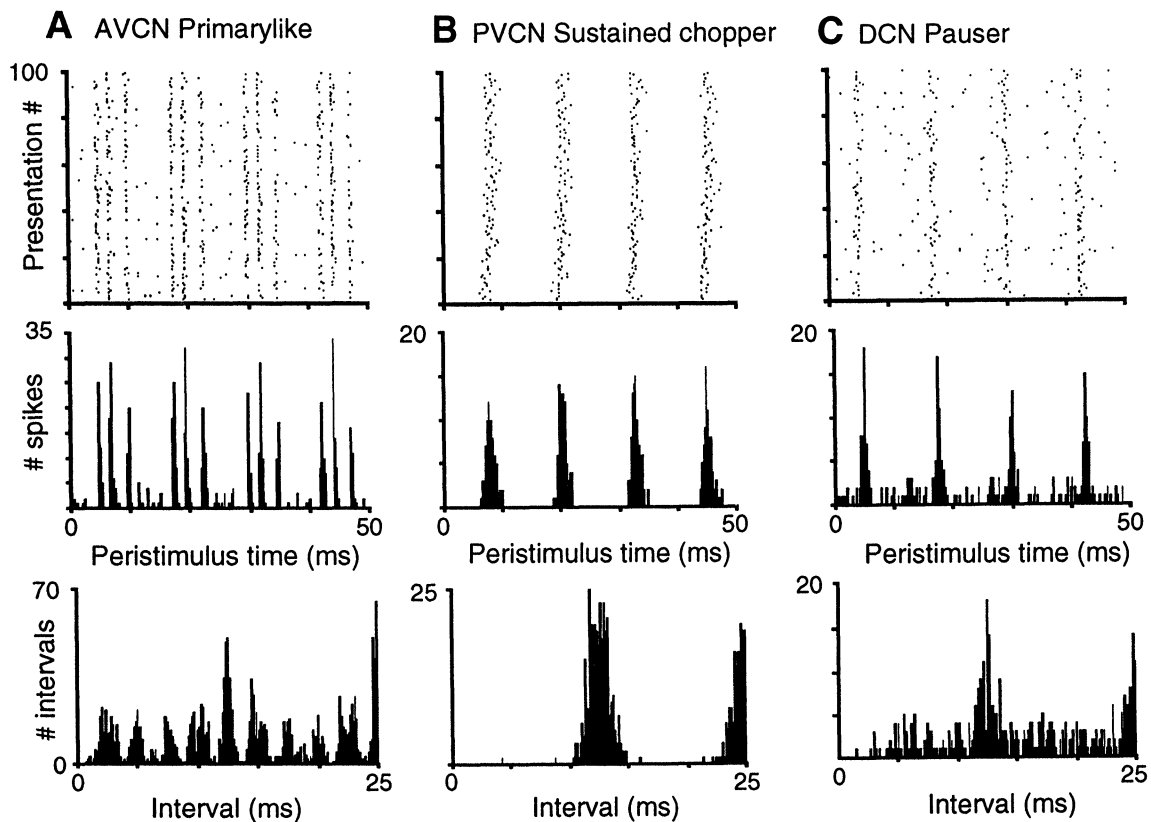
Fig. 6: Responses of three units in the cochlear nucleus to 100 presentations of a single-formant vowel ( F_0=80 Hz, F_1=640 Hz, BW=50 ) at 60 dB SPL. Units were classified according to their PSTH response to short tone bursts at CF. A. Dot-raster, PSTH, and all-order interval histogram for a primarylike unit in antero-ventral cochlear nucleus (AVCN), CF=400 Hz. B. Response of a sustained chopper unit in posterior-ventral cochlear nucleus (PVCN), CF=1.5 kHz. C. Response of a pauser unit in dorsal cochlear nucleus (DCN), CF=4.4 kHz.
