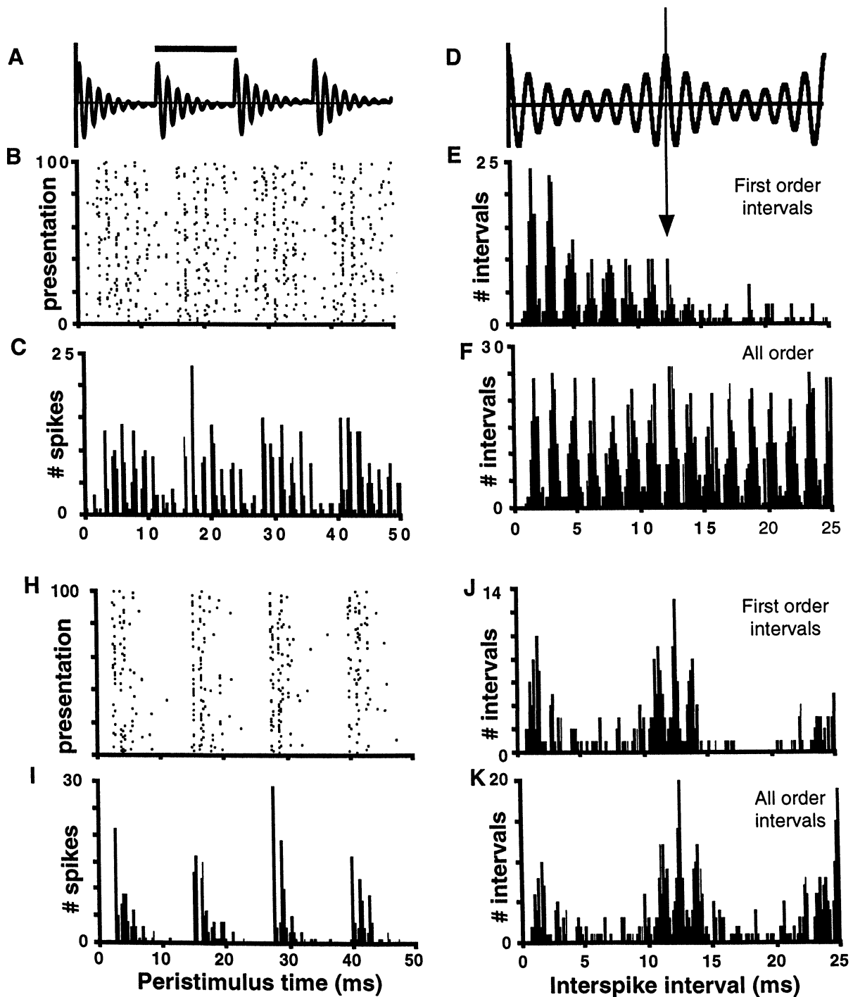
Fig. 4: Responses of two auditory nerve fibers with different CF's to 100 presentations of a single formant vowel, 60 dB SPL. A-F. Unit 25-19, CF = 950 Hz, near the formant region. H-K. Unit 25-91, CF = 2.1 kHz, well above the formant region. A. Vowel waveform. Fundamental period 1/F_0 (line) is 12.5 ms, F_0 = 80 Hz. B. Dot raster display of individual spike arrival times. C. Peristimulus time histogram of spike arrival times. D. Stimulus autocorrelation function. Vertical line indicates fundamental period, 1/F_0 = voice pitch. E. Histogram of first-order interspike intervals (between consecutive spikes). Arrows indicate intervals near the fundamental/pitch period. F. Histogram of all-order intervals (between both consecutive and nonconsecutive spikes). H-K. Corresponding histograms for the second fiber.
