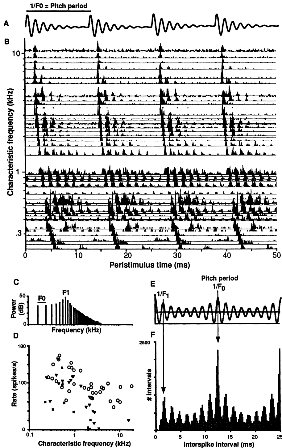
Fig. 3: Auditory nerve response to a single-formant vowel. A. Vowel waveform. A strong, low voice pitch is heard corresponding to the fundamental period, 1/F_0=12.5 ms. B. Peristimulus time histograms of 51 cat auditory nerve fibers to 100 presentations at 60 dB SPL, arranged by characteristic frequency (CF). C. Power spectrum of the vowel (logarithmic frequency scale). The fundamental frequency, ( F_0=80 Hz = frequency spacing of harmonics) and the formant frequency ( F_1 = 640 Hz = spectral peak) are indicated. Bandwidth = 50 Hz. D. Discharge rates as a function of CF and spontaneous rate (SR) (circles, high SR; triangles, medium SR; crosses, low SR). E. Stimulus autocorrelation function. Arrows indicate formant period 1/F_1 and fundamental period 1/F_0 . F. Population-interval distribution formed by summing all-order intervals from all fibers.
