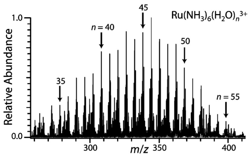
Figure 1. ESI mass spectrum of \sim 2 mM aqueous \text{Ru}(\text{NH}_3)_6^{3+} showing hydrated clusters, \text{Ru}(\text{NH}_3)_6(\text{H}_2\text{O})_n^{3+} , with n indicated in the figure.
