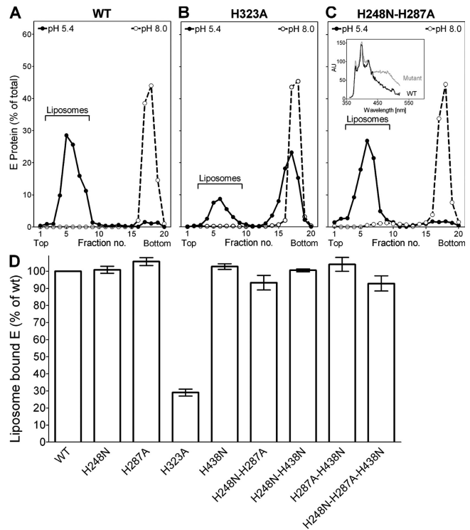
Figure 4. Acidic pH-induced coflotation of WT and mutant RSPs with liposomes. RSPs were incubated with liposomes at pH 5.4 (solid lines) and 8.0 (dotted lines), back-neutralized, and then subjected to centrifugation in sucrose step gradients. The gradients were fractionated, and the amount of E protein in each fraction was determined by a quantitative four-layer ELISA. The top fractions containing RSPs coflotated with the liposomes are indicated by a bracket. (A–C) Representative examples of the analysis of the step gradients obtained with WT (A) and the fusion-negative mutants H323A (B) and H248N-H287A (C). The inset in C shows the fluorescence spectrum of the coflotated fractions of the mutant (gray) relative to those of the WT (black) from experiments using pyrene-labeled RSPs. AU, arbitrary units. (D) Extent of acidic pH-induced coflotation of E with liposomes obtained with mutant RSPs relative to the WT (set at 100%). The data are the means from at least two independent experiments; the error bars represent the standard errors of the means.
