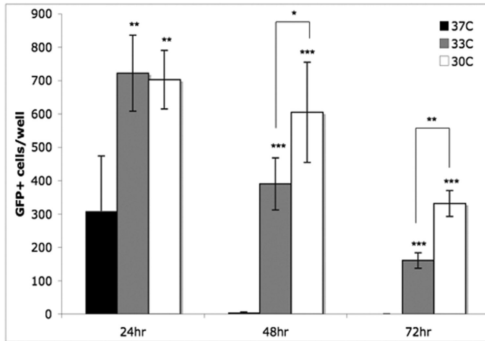
Figure 3. Survival of OSNs in culture is prolonged by decreased incubation temperature
