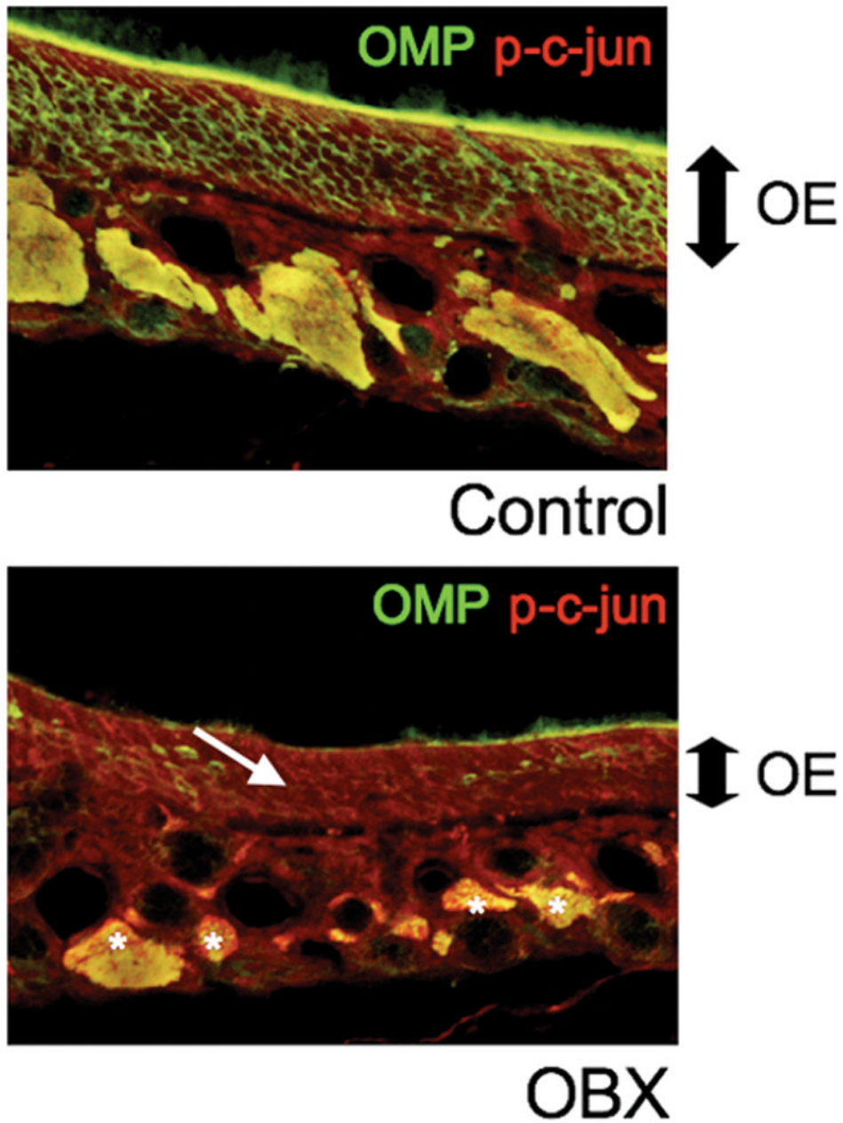
Figure 6. Phosphorylation of c-jun increases in vivo following removal of the olfactory bulb Tissue from the olfactory epithelium of an adult mouse was fixed after a 5-day survival period following unilateral olfactory bulbectomy (OBX) in which one lobe of the olfactory bulb was removed, and the opposite side was left in tact as an internal control. On the unoperated side (top panel), the neuronal layer of the epithelium remains thick as demonstrated by OMP labeling, while the operated side (lower panel) has decreased in thickness as sensory neurons have died. Concurrently, the level of c-jun phosphorylation has increased on the operated side in the neuronal layer (arrow) and in the axons bundles (asterix); p-c-jun levels remain low on the unoperated side.
