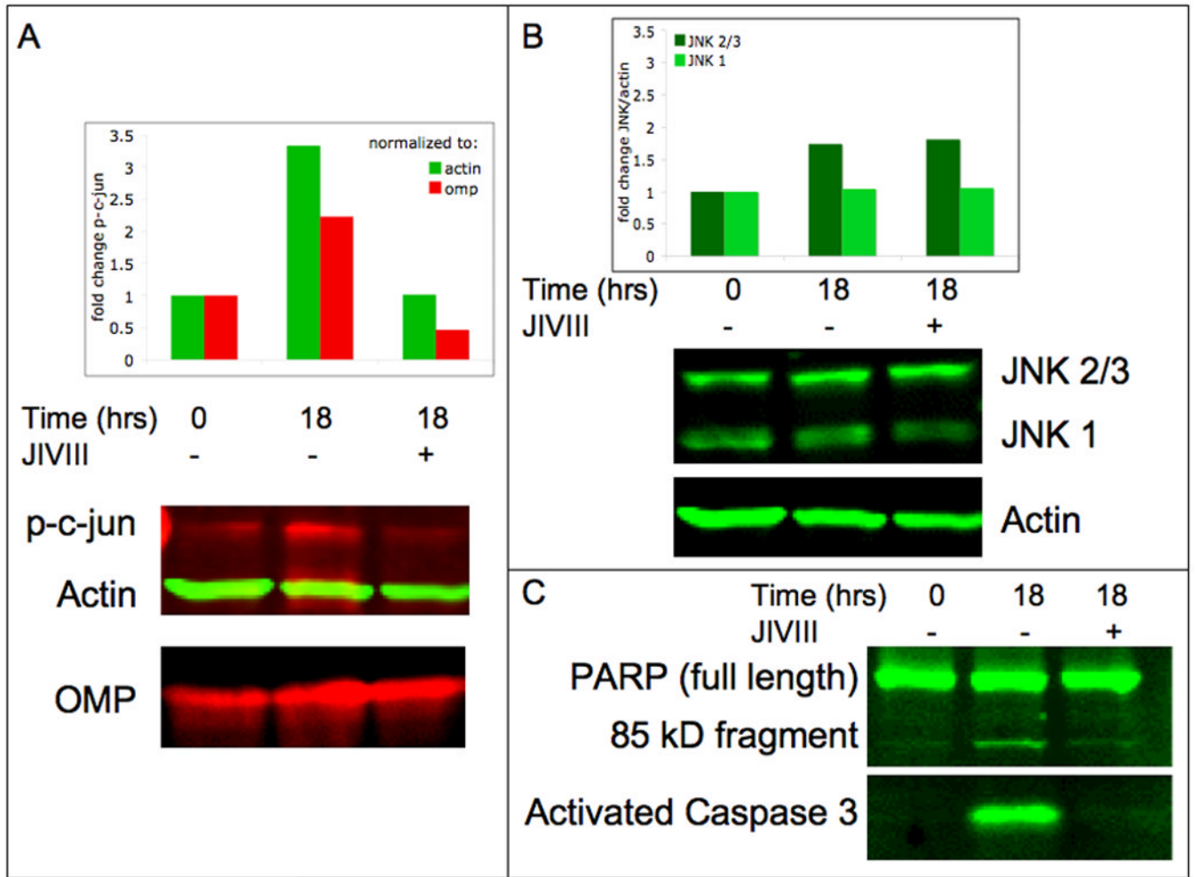
Figure 5. JNK inhibition prevents both c-jun phosphorylation and caspase-3 activation in cultured OSNs
