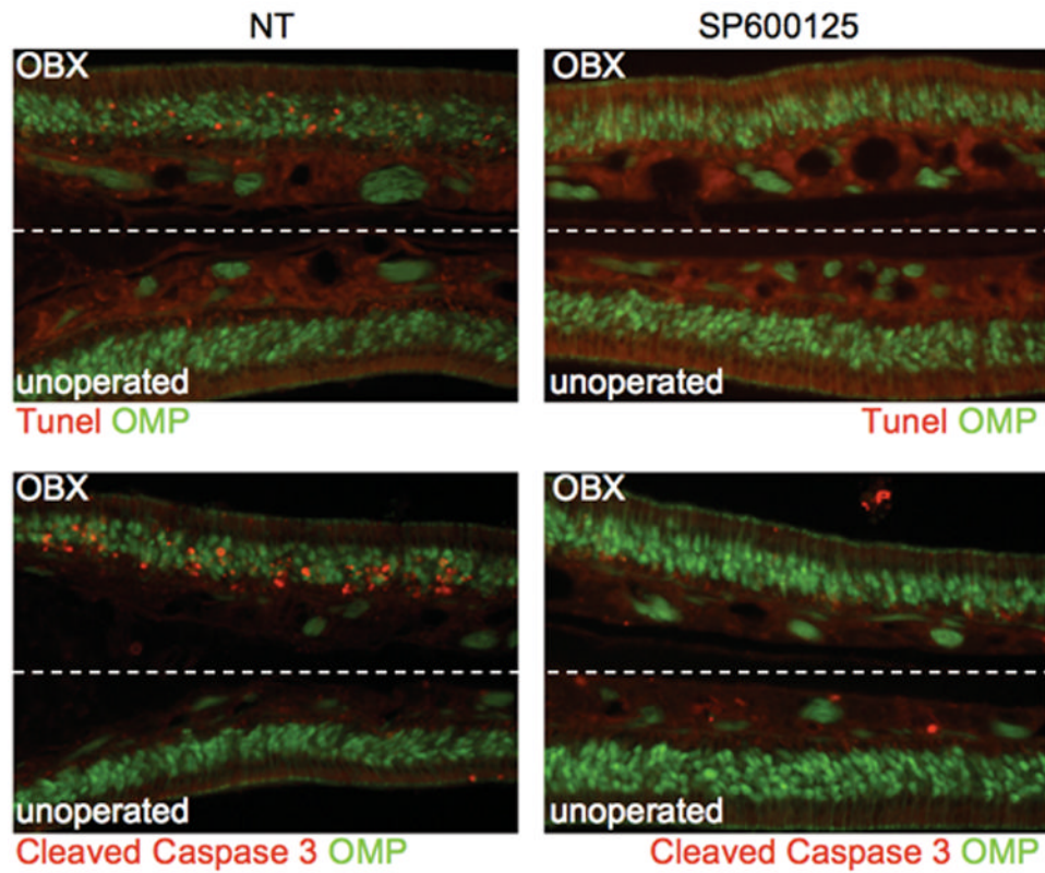
Figure 7. Inhibition of JNK activity suppresses OSN death following OBX
