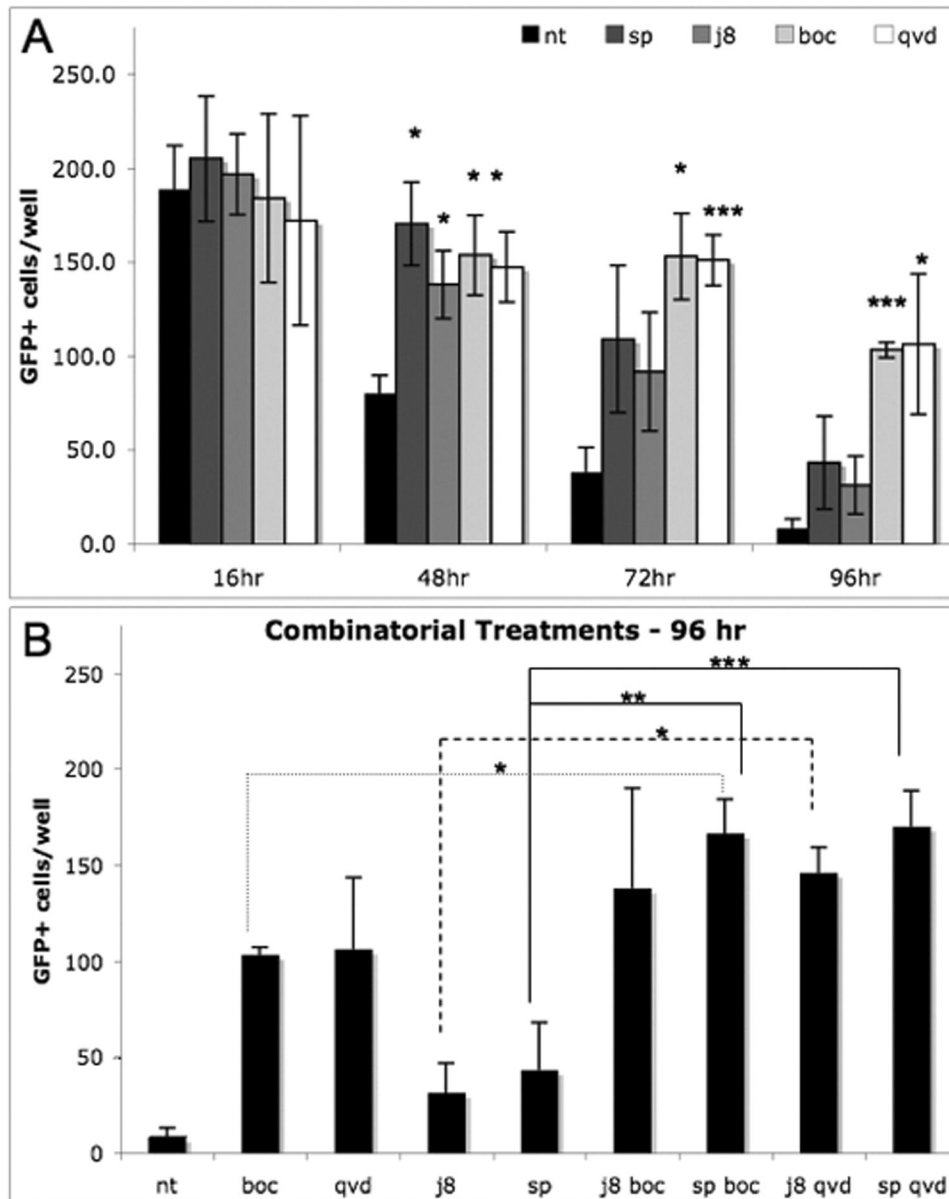
Figure 4. Pan-caspase and JNK inhibitors delay death of OSNs
