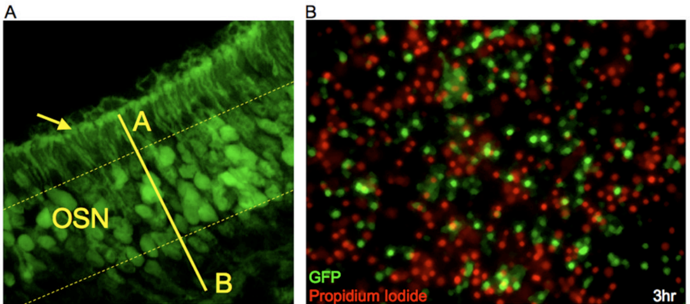
Figure 1. GFP is expressed in mature olfactory sensory neurons of OMP-GFP knock-in mice (a) Coronal section through the olfactory epithelium of a transgenic adult mouse in which the transcription of GFP has been placed under the control of the OMP promoter. GFP expression is visible in the soma of neurons within the mature neuronal layer, labeled OSN between dashed yellow lines, and in their dendritic knobs (arrow) that protrude from the apical surface of the epithelia (A = apical; B = basal). (b) Dissociated cells from the olfactory epithelium of an adult OMP-GFP mouse. Mature sensory neurons retain GFP expression (green) while they are alive, and dead or dying cells within the culture stain positive for propidium iodide (PI, red) and no longer express GFP. While there are high numbers of both PI+ cells and GFP+ cells, there is very little overlap of the two labels, indicating that OSNs no longer express GFP as they are dying: of 310 GFP+ cells counted, only 1.6% of those GFP+ cells stained positive for PI. Therefore the GFP signal can be used as an indicator of live mature OSNs.
