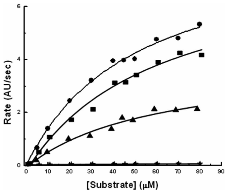
Figure 2. The enzymatic activities of wild type 3CL pro (●), S139A (■), S144A (▲), and S147A (◆) were determined at 25°C with an enzyme concentration of 1 μM in 10mM NaCl, 10mM NaPi, 1mM EDTA, 1mM TCEP (pH 7.4). The initial velocity, which was measured as arbitrary fluorescence units per second, is plotted as a function of substrate concentration.
