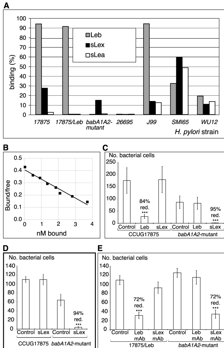
Fig. 3. H. pylori binds sialylated antigens. (A) H. pylori strains and mutants (14) were analyzed for binding to different ^{125}\text{I} -labeled soluble fucosylated and sialylated (Lewis) antigen-conjugates [RIA in (14)]. The bars give bacterial binding, and conjugates used are given in the diagram. (B) For affinity analyses (16), the sLex conjugate was added in titration series. The babA1A2 mutant was incubated for 3 hours with the s(mono)Lex conjugate to allow for equilibrium in binding, which demonstrates an affinity ( K_a ) of 1 \times 10^8 \text{ M}^{-1} . (C) Adherence of strain 17875 (sLex and Leb-antigen binding) and babA1A2 mutant to biopsy with inflammation and H. pylori infection, as scored by the number of bound bacteria after pretreatment with soluble Leb (Fig. 1, E and F) or sLex antigen (Fig. 1, H and I) (14). The Leb antigen reduced adherence of strain 17875 by >80%, whereas the sLex antigen abolished adherence of the babA1A2 mutant. (D) Adherence of strain 17875 and babA1A2 mutant to biopsy of Leb mouse gastric mucosa was scored by the number of bound bacteria after pretreatment with sLex conjugate. Adherence by the babA1A2 mutant was abolished (Fig. 2A, vi), while adherence by
