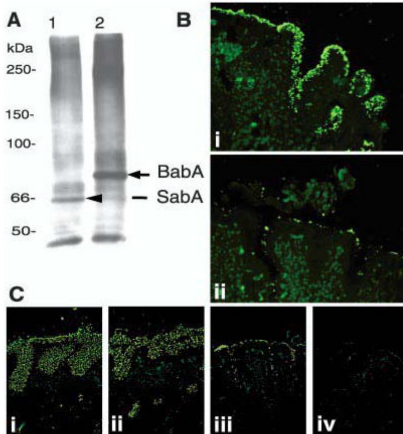
Fig. 5. Retagging of SabA and identification of the corresponding gene, sabA . After contact-dependent retagging (of the babAIA2 mutant) with crosslinker labeled sLex conjugate, the 66-kDa biotin-tagged adhesin SabA [(A), lane 1] was identified by SDS–polyacrylamide gel electrophoresis/steptavidin-blot, magnetic-bead-purified, and analyzed by MS for peptide masses (14). As a control, the Leb conjugate was used to retag 17875 bacteria, which visualized the 75-kDa BabA adhesin [(A), lane 2] (4). (B) The J99/JHP662::cam ( sabA ) mutant does not bind the sLex antigen but adheres to human gastric epithelium [(B), i], due to the BabA-adhesin, because pretreatment with soluble Leb antigen inhibited binding to the epithelium [(B), ii]. (C) The J99 wild-type strain (which binds both Leb and sLex antigens) [(C), i] and the J99 sabA mutant (which binds Leb antigen only) [(C), ii] both exhibit strong adherence to the gastric mucosa. In comparison, the J99 babA mutant binds by lower-affinity interactions [(C), iii], while the J99 sabAbabA mutant, which is devoid of both adherence properties, does not bind to the gastric mucosa [(C), iv].
