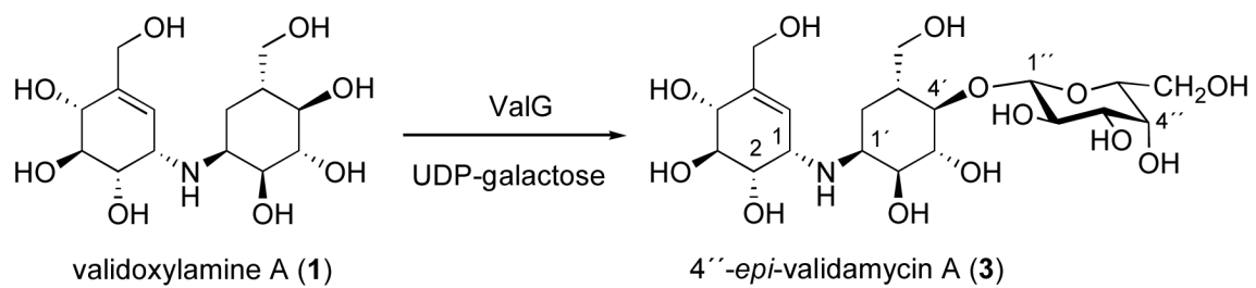
Figure 2. Bioconversion of 1 to 3 using the glycosyltransferase ValG.
