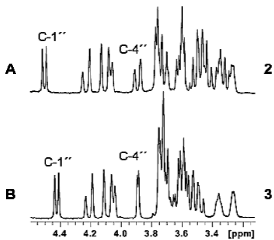
Figure 3. Partial ^1\text{H} NMR spectra of validamycin A (2) and 4'' - epi -validamycin A (3).
