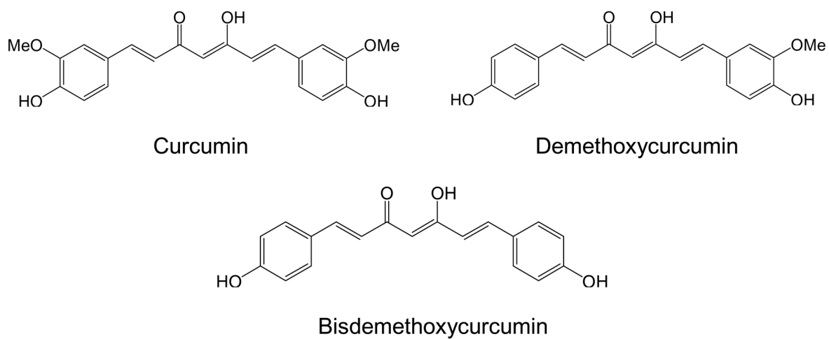
Figure 1. Structures of curcuminoids studied.
