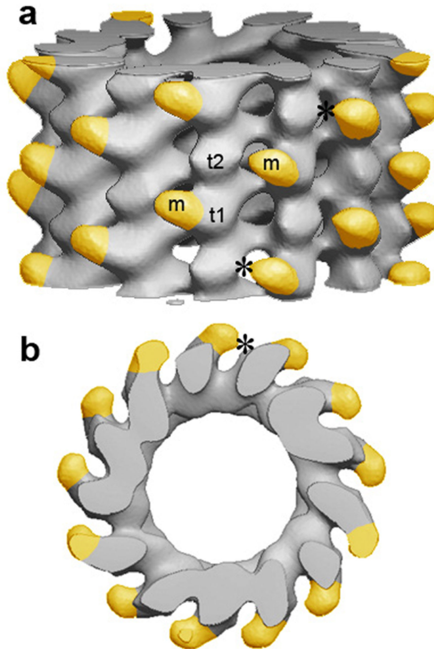
Figure 4. Three-dimensional reconstruction of Mal3-143-decorated A-lattice microtubule. (a) Side view of the microtubule. (plus end upward). (b) End-on projection seen from the plus end. Mal3 density is highlighted in yellow. Asterisks show where Mal3 (m) almost touches a tubulin subunit in the neighboring protofilament. Subunits t1 and t2 may represent \alpha - and \beta -tubulin, respectively.
