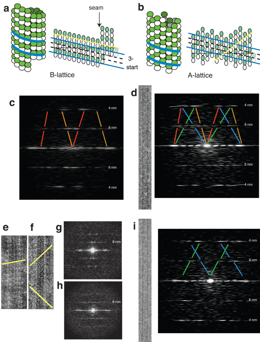
Figure 3. Microtubules assembled with Mal3 show mixed lattices. (a,b) Diagrams of microtubules with A- and B-lattices of tubulin heterodimer subunits, represented both as three-dimensional microtubules and as opened-out sheets. White subunits, \alpha -tubulin; green subunits, \beta -tubulin; blue lines, the direction of the 3-start family of helices, common to both lattices, that arises because subunits in adjacent longitudinal protofilaments are staggered by 0.9 nm; yellow lines, the directions of the decoration patterns, different on both lattices, as shown in e and f . (c) Diffraction pattern from a cryo-EM image of a pure tubulin microtubule decorated with kinesin head domains. Red and orange lines show the B-lattice
