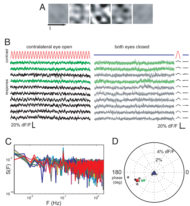
Fig. 2. Measuring cell responses to monocular visual stimulation. (A) Contrast modulated stochastic noise visual stimulus. A grayscale movie, modulating sinusoidally between zero and maximal contrast with a 10-s period, was presented separately to each eye (Movie S1 (AVI)). The noise stimulus contained spatial and temporal components tailored to the selectivity of mouse primary visual cortical neurons. (B) Example cellular calcium signal traces from 10 simultaneously recorded neurons during 30 cycles of the noise stimulus presented to one eye only (Left), or with both eyes occluded (Right). Recordings from inhibitory neurons are in green. Time average of 30 cycles plotted for each stimulation condition (far right) shows a periodic response to monocular stimulation in all cells. Scale bars are 20 s (Left) and 10 s (Right). (C) Power spectra of responses to contralateral stimulation show a peak at the fundamental frequency of contrast modulation. (D) Responses to visual stimulation are well separated from nonstimulated condition. Shown is a polar plot of the phase and amplitude of the best-fitting sinusoid of period 10 s for each of the cells above in stimulated (open circles) and unstimulated control (filled circles) conditions. Red and blue asterisks indicate the mean response across cells for the stimulated and nonstimulated conditions, respectively. Green circles indicate inhibitory cell responses.
