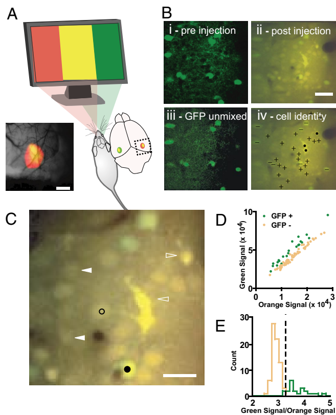
Fig. 1. Identifying inhibitory neurons in the binocular primary visual cortex. (A) Intrinsic signal optical imaging reveals the binocular zone of mouse primary visual cortex. Response maps to contralateral eye (in red) and ipsilateral eye (in green) visual stimulation are superimposed. The region of binocular overlap appears as yellow. Subsequent calcium indicator labeling and recording were targeted to the medial half of the mapped binocular region, corresponding to primary visual cortex. (Scale bar: 0.8 mm.) (B) Fluorescent signals from GFP-positive inhibitory cells and bulk-loaded calcium indicators are separable. Single plane imaged in two color channels from visual cortex of a mouse line expressing GFP in inhibitory neurons shown before (i) and after (ii) the extracellular loading of calcium indicator. GFP-positive cells stand out from neuropil and GFP-negative cells. (iii) GFP fluorescence is linearly separable from calcium indicator fluorescence after indicator loading. (iv) Merged image from ii annotated with + symbols for excitatory neurons, - for inhibitory neurons, and ● for astroglia. (Scale bar: 40 \mu\text{m} .) (C) Selection of pixels used to measure responses of individual neurons. Circular pixel selections 4 \mu\text{m} wide (examples shown in black; filled is inhibitory and open is excitatory) were drawn within the boundaries of each cell body to guarantee exclusion of neuropil signal contamination. Cell bodies that were poorly sectioned (filled triangles) as well as morphologically identified astroglia (open triangles) were excluded from analysis. (Scale bar: 20 \mu\text{m} .) (D and E) Neurons identified as GFP-positive before indicator loading (green) are discriminated from GFP-negative neurons (orange) by the ratio of green to orange fluorescence intensity. A discriminator partitions the GFP-positive from GFP-negative neurons (dashed line in E).
