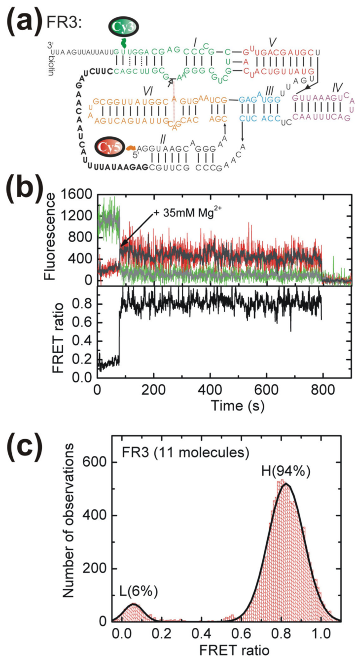
Fig. 5. Docking of the alternatively connected, catalytically active FR3 ribozyme. (a) Secondary structure of the FR3 ribozyme showing its alternative connectivity (bold) to the downstream stem-loop I substrate. Fluorophore labeling sites were chosen similar to those of WT in Fig. 2. (b) Example trace of a FR3 molecule. The raw Cy3 (donor) and Cy5 (acceptor) intensities are shown along with the non-linear averaged data (Haran, 2004) in gray. The FRET ratio calculated as I_A/(I_A + I_D) for the averaged data is shown in black. (c) An aggregate FRET ratio histogram for data points after addition of 35 mM Mg 2+ is well described by a gaussian distribution of two states.
