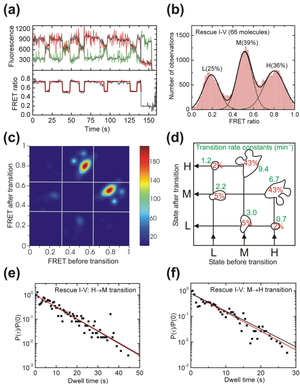
Fig. 4. Single molecule FRET analysis of the Rescue I-V ribozyme. (a) Representative FRET time trace of a Rescue I-V molecule. The raw Cy3 donor and Cy5 acceptor fluorescence signals are green and red, respectively. Superimposed in gray are the data after applying a non-linear filter as described. 38 The FRET ratio (black trace below) is calculated from the filtered data as I_A / (I_A + I_D) and reveals three distinct states in Hidden Markov modeling (HMM, red line). (b) An aggregate FRET histogram of 66 Rescue I-V molecules shows Gaussian distributions for three states with FRET values of \sim 0.80 (H), \sim 0.51 (M) and \sim 0.19 (L) and the indicated abundances. (c) Transition density contour map from HMM analysis 54 of all transitions for 62 well defined Rescue I-V molecules. (d) Relative contributions and mean rate constants of
