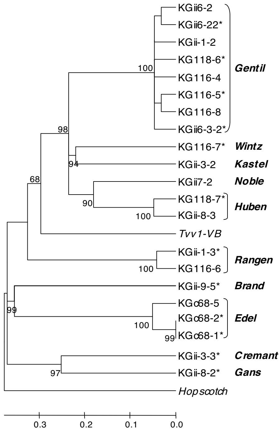
Figure 1 Classification of the 21 novel full-length retrotransposon sequences into 10 families. The Neighbor-Joining tree is based on the multiple sequence alignment of amino acid sequences between reverse transcriptase domains I and VII using the Poisson distance model. * Insertions displaying perfect target duplication sites. Ty1/copia retrotransposons Tw1 from grapevine and Hopscotch from maize (acc. n° U12626) were added as references. Bootstrap values greater than 60% are shown on the tree.
