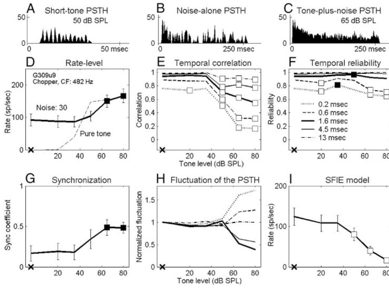
FIG. 2. Responses of a chopper unit to a short tone (25 ms, 50 dB SPL), long tones (250 ms), noise alone (250 ms), or tones plus noise (250 ms). A : PSTH for responses to the short tone at CF. Bin width = 0.5 ms. B–I : tone-in-noise responses. B : PSTH for noise at 30 dB SPL spectrum level. Bin width = 2 ms. C : PSTH for noise in B plus a 65 dB SPL tone. Bin width = 2 ms. D : masked rate-level functions for a 250-ms CF tone and for tone plus noise. E : temporal correlation measured with different temporal-analysis windows. F : temporal reliability measured with different temporal-analysis windows. G : synchronization coefficient to tone. H : PSTH fluctuation measured with different temporal-analysis windows. I : rate-level function of SFIE model. All filled squares indicate significant increase, and all open squares indicate significant decreases ( P < 0.05 or d' \geq 1 ). X on the abscissa indicates responses to noise alone. G309u9: CF = 492 Hz, SR = 0 sp/s. Pure-tone rate threshold in quiet = 22 dB SPL (same neuron as in Fig. 1). Fifty trials per stimulus condition. Error bars are SD.
