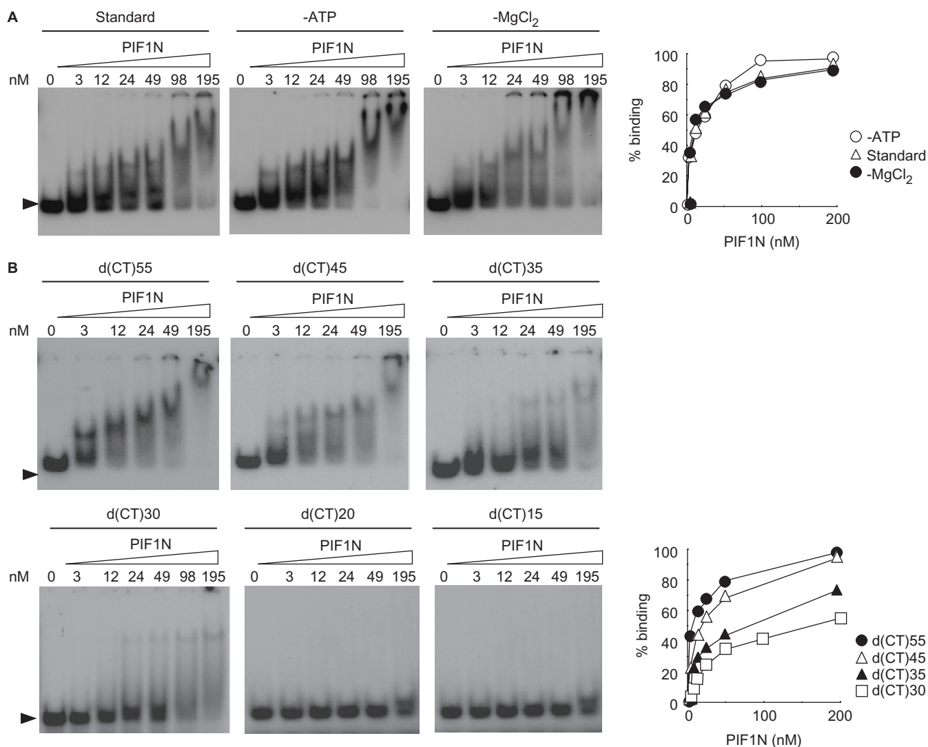
Figure 4. EMSA of PIF1N for binding to ssDNA. (A) Titration of PIF1N under different conditions. The 5'- 32 P labeled oligonucleotide, d(AC)60, was incubated with the shown concentrations of PIF1N, omitting ATP or \text{MgCl}_2 as indicated. Arrowheads indicate the positions of free DNA. The quantified data are shown graphically. (B) Binding ability of PIF1N to different sizes of oligonucleotides. Experiments were performed using indicated oligonucleotides as substrates under standard reaction conditions in the absence of ATP. The quantified data are shown graphically. The errors in the experiments were <10%.
