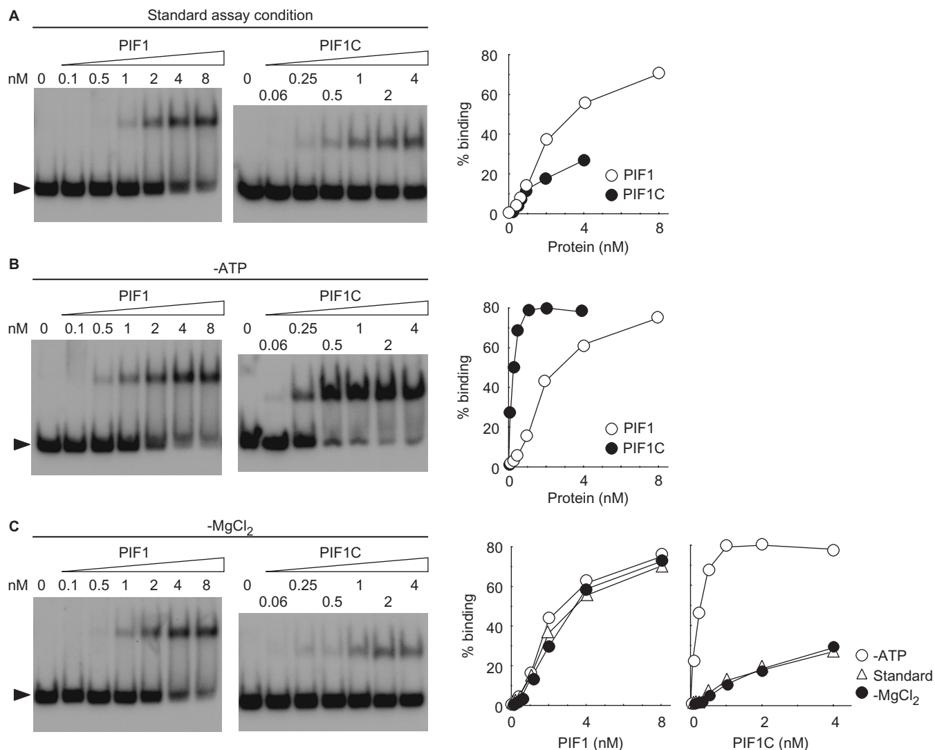
Figure 3. EMSA of PIF1 and PIF1C for binding to ssDNA. (A) EMSA of ssDNA binding to PIF1 and PIF1C under standard reaction conditions. The 5' - ^{32} P labeled oligonucleotide, d(AC)60, was incubated with the indicated concentrations of PIF1. Arrowheads indicate the positions of free DNA. The quantified data are shown graphically. (B) EMSA in the absence of ATP. Experiments were performed as described in (A). The quantified data are shown graphically. (C) EMSA in the absence of MgCl_2 . Experiments were performed as described in (A). The quantified data are shown graphically together with data from (A) and (B). The errors in the experiments were <10\% .
