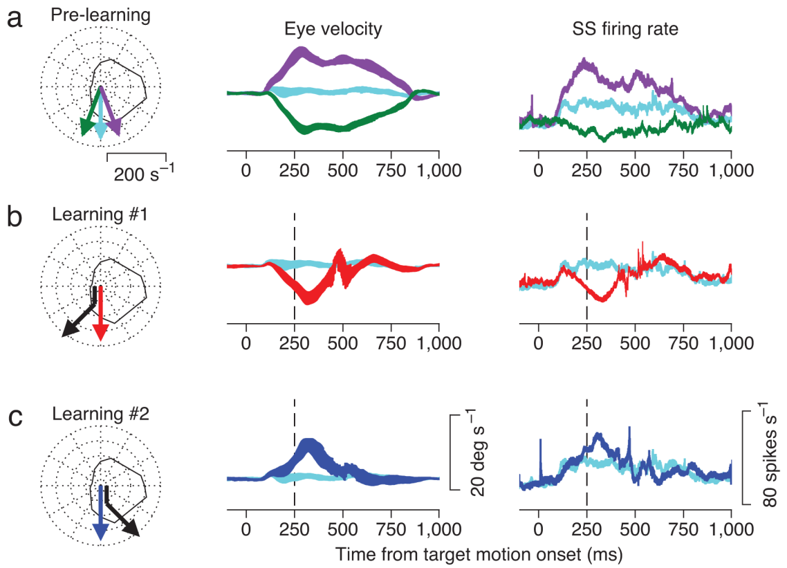
Figure 2. Effects of learning on responses of one Purkinje cell. From top to bottom, the three rows show the control block, and the learning blocks in the off- and on-direction of the Purkinje cell. In the left column, the colored arrows show different target motions and the black continuous curve shows the direction tuning for the Purkinje cell. The middle and right columns show eye velocity and simple spike firing rate during probe trials. The colors of the traces refer to the different target trajectories indicated by the colored arrows in the polar plots. For ease of comparison, the light blue traces in b and c replot the pre-learning data for downward target motion from a . The ribbons show the mean \pm 1 SEM of eye velocity and firing rate.
