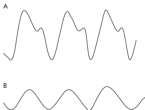
Figure 1 (A) Normal arterial pressure waveform and (B) over-damped arterial pressure waveform, due to partially blocked arterial cannula or air bubbles in circuit.
