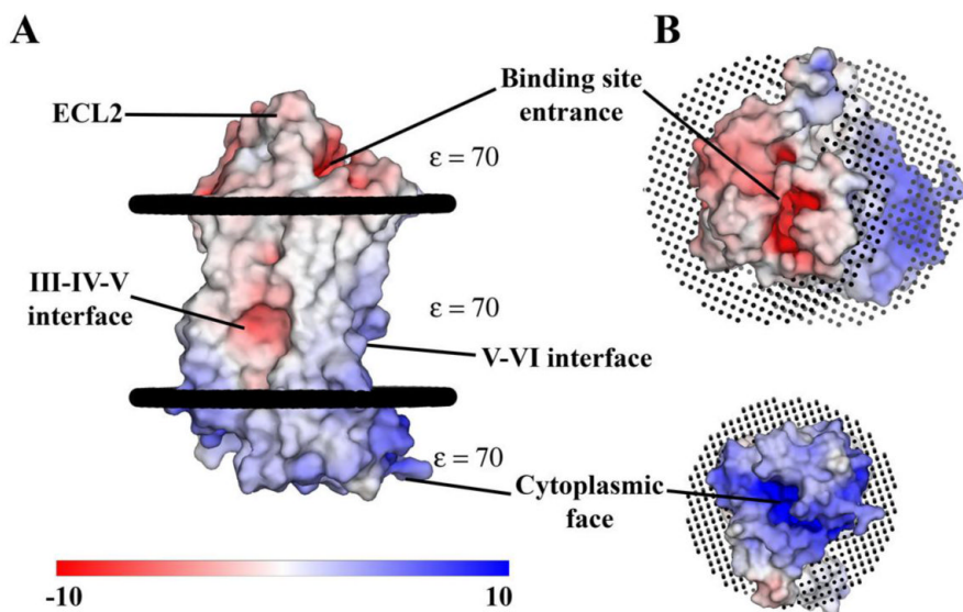
Figure 3. Surface representation of \beta_2 AR colored by calculated charge from red ( -10 k_B T/e_c ) to blue ( +10 k_B T/e_c ) using a dielectric constant of 70. A. Three main areas of interest are indicated. The binding site cleft is negatively charged as is a groove between helices III, IV and V. The third region is an overall positive charge in the region of the ionic lock and DRY motif on the cytoplasmic face. The overall result is a highly polarized molecule that may utilize its negative charge to facilitate binding of catecholamine ligands. The presence of a negative charge in the groove between helices III, IV and V is unexpected as it is in the middle of the lipid membrane. This charge may be partially derived from the presence of an unpaired glutamate at position 122 3,41 . The effective charge in this region is likely greater than shown here due to its location in the low dielectric environment of the lipid membrane. B. View rotated 90^\circ from A. Showing both the negatively charged binding site cleft (top) and positively charged cytoplasmic face (bottom). Poisson-Boltzmann electrostatics were calculated using the program APBS (53) as implemented in Pymol (75). Pymol was used exclusively in the preparation of all figures.
