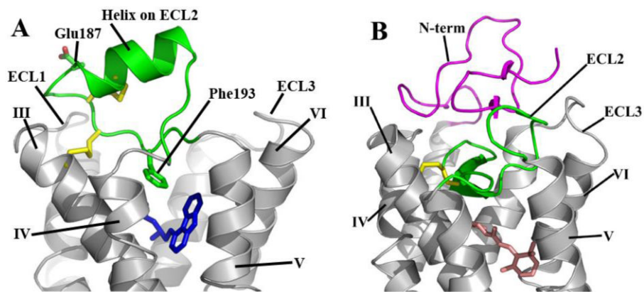
Figure 4. Comparison of the extracellular sides of \beta_2 AR-T4L and rhodopsin. A. The N-terminus is missing from the experimental density in the \beta_2 AR-T4L structure and is not shown. ECL2 is shown in green and contains a short \alpha -helix and two disulfide bonds (yellow). The intraloop disulfide bond constrains the tip of ECL2 which interacts with ECL1. The second disulfide bond links ECL2 with helix III. There is one interaction between ECL2 and carazolol (blue) through Phe193 5,32 . The entire loop is held out of the ligand binding site by a combination of the rigid helical segment and the two disulfide bonds. B. In contrast, ECL2 (green) in rhodopsin assumes a lower position in the structure that occludes direct access to the retinal-binding site and forms a small \beta -sheet in combination with the N-terminal region (magenta) directly above the bound retinal (pink).
