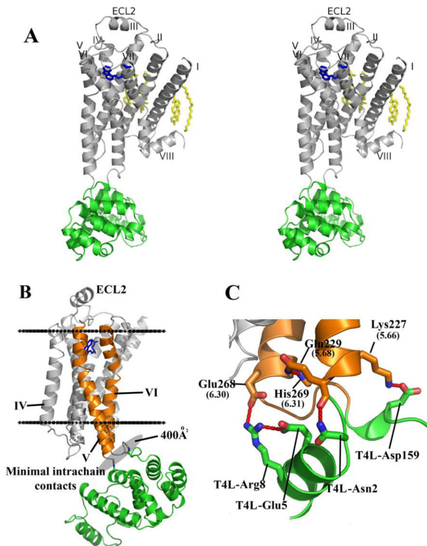
Figure 1. Overall fold of the \beta_2 AR-T4L fusion with its predicted orientation in the plasma membrane and key intramolecular interactions. A. Stereoview of the overall fold of \beta_2 AR-T4L. The receptor and T4L are colored gray and green, respectively. Carazolol is colored blue and the lipid molecules bound to the receptor are colored yellow. B. The receptor is aligned to a rhodopsin model that was positioned in a lipid membrane (boundaries indicated by horizontal black lines) as found in the orientations of proteins in membranes (OPM) database (74). T4L is fused internally into the third intracellular loop of \beta_2 AR and maintains minimal intramolecular packing interactions by tilting away from the receptor. C. Specific intramolecular interactions between \beta_2 AR and T4L are represented.
