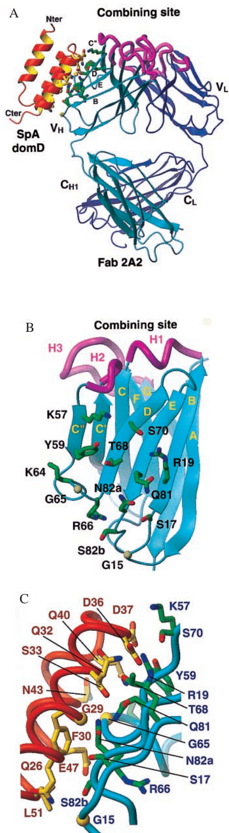
Fig. 1. Schematic representation of the complex between SpA domain D and Fab 2A2 from a human IgM. (A) Side view showing SpA domain D (red) bound to the framework region of the Fab heavy chain (cyan). The V_L domain, which is not involved in this interaction, is shown in dark blue. The CDR loops as defined by Chothia and Lesk (33) are highlighted in magenta. (B) Ribbon representation of the V_H region of Fab showing the positions of the residues that interact with domain D. (C) Schematic diagram detailing the residues of
