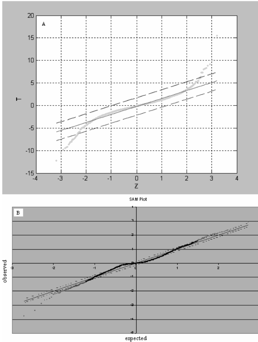
Fig. 1. Identification of the genes significantly differentially expressed. Panel A is a plot of T-values vs Z-values based on the observed data of 3000 genes in two samples each consisting of 12 rat individuals in response to stroke where estimates of Z-values were obtained by use of the RS approach. Panel B is plot of observed T vs expected T (Z) in SAM. The simulated data set was comprised of 30% expression noises following gamma distribution and 70% following normal distribution where expression levels of 3000 genes in two samples each consisting of 12 replicates were simulated using one set of the observed sample means and two sets of the observed sample variances, and treatment effect values of G=10R (for 30% of the genes) where R is a random uniform variable over (0, 1] .
