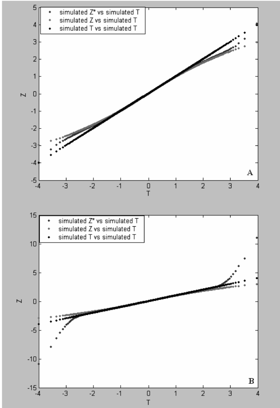
Fig. 3. Plots of Z-values vs T-values. The observed Z-value (the b line) and simulated Z-value (the c line) were obtained by the permutation approach (panel A) and the RS approach (panel B). The observed microarray data of 3000 genes were obtained in two samples each consisting of 12 rat individuals. The first set of the simulated microarray data were produced using the pseudorandom generator and one set of 3000 observed means and two sets of 3000 observed variances where no gene was not given a treatment effect value. The simulated T- values (the a line) were a set of 3000 null scores produced from 100 repeated simulations of the first set of the simulated data (see text).
