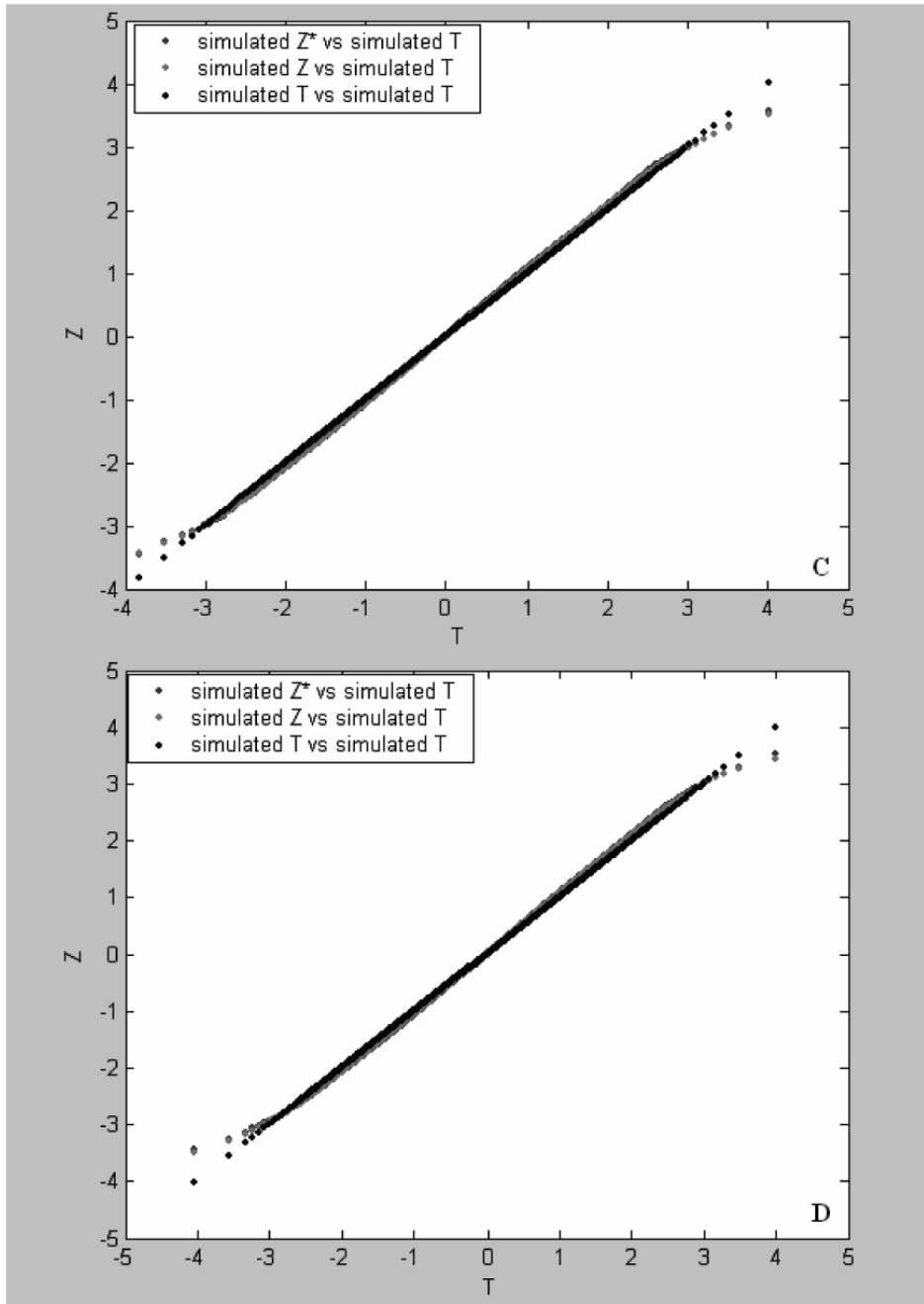
Fig. 4. Plots of Z-values vs T values. The simulated Z-values were obtained from the first (the c line), second (the b lines in panels A and C) and third (the b lines in panels B and D) sets of the simulated data of 3000 genes, respectively. In the first, second, and third simulation sets, treatment effect values of G=0R , 10R and 30R were randomly assigned to 30% of the genes, respectively, where R is a random variate in the uniform distribution (>0,1] (see text for simulation). The simulated T-values (the a line) were a set of 3000 null scores (see text). The results shown in A and B were obtained by the permutation approach and those shown in panels C and D were based on the RS approach.
