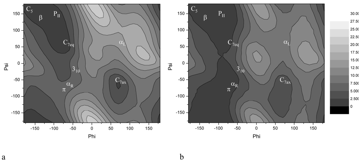
Figure 1. Ramachandran diagram for the alanine dipeptide in vacuo (left panel) computed using the CHARMM27 potential function, and including solvent water (right panel) computed using the finite difference Poisson Boltzmann (PB) implicit solvent model. Conformation regions are indicated on the map.
