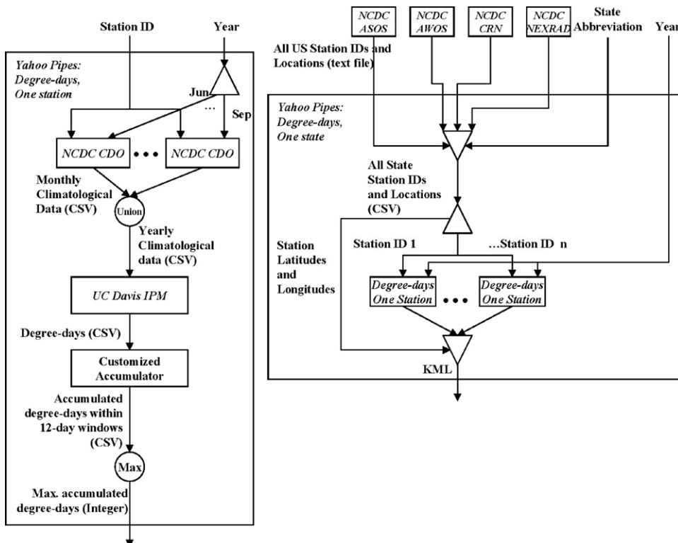
Figure 1. Schematic diagram illustrating how the developers combined different web-based data and analytical services to produce the application.
