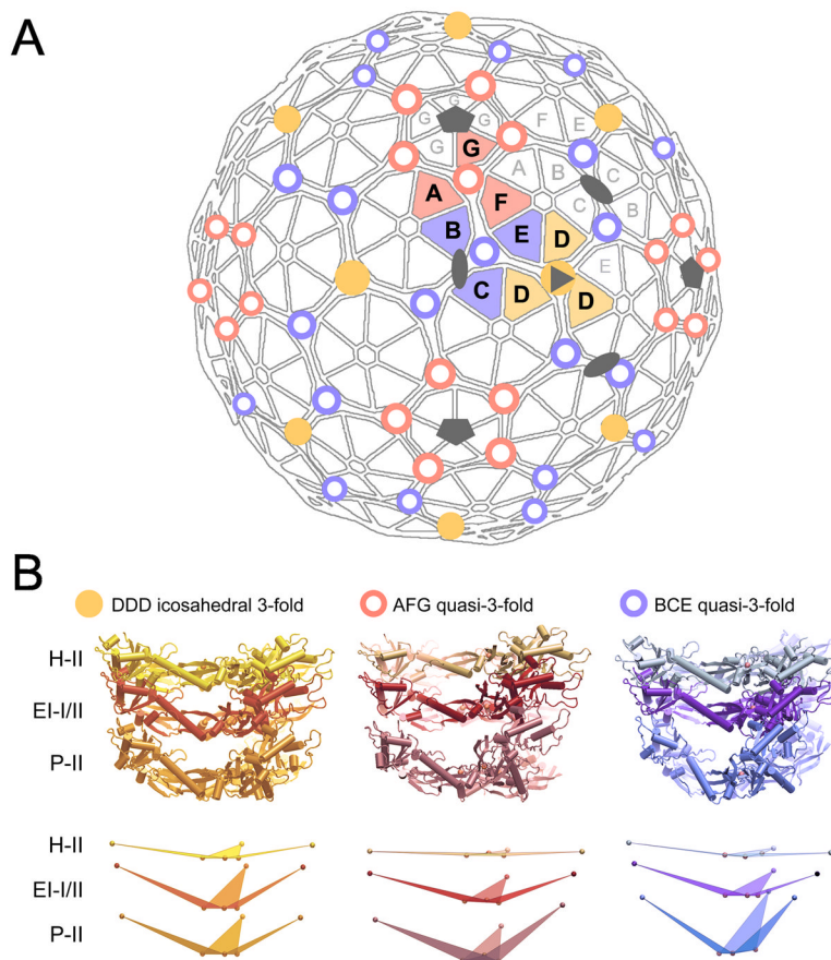
Figure 5. Hinges in HK97 capsid lattice
