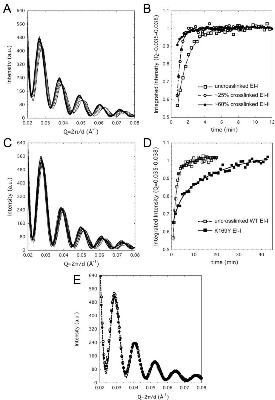
Figure 3. Time-resolved SAXS following reneutralization-induced conversion of EI-I/II to Balloon particles
