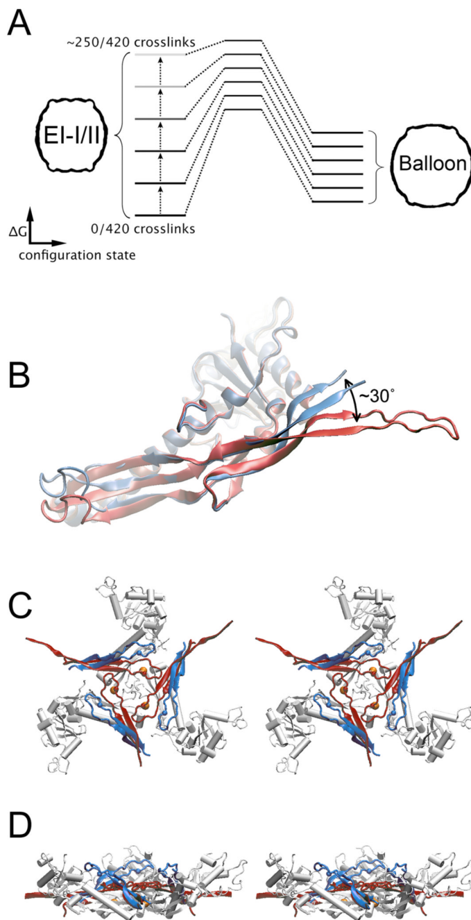
Figure 6. Crosslink-dependent E-loop bending spring-loads the 3-fold and quasi-3-fold hinges and switches the conformational balance towards Balloon
