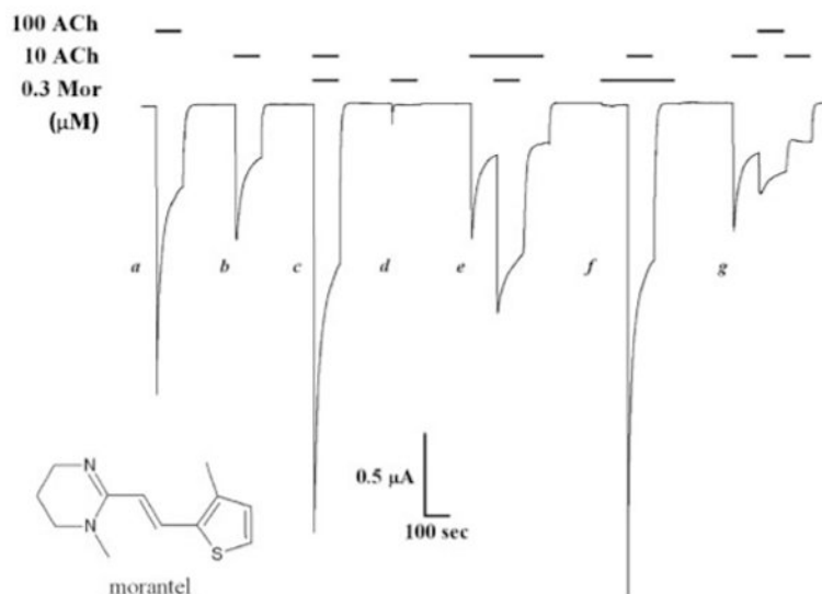
Fig. 1. Morantel does not affect desensitization. A sample continuous current trace for an oocyte expressing \alpha_3\beta_2 receptors is shown. Drug applications were for 100 or 300 s when either ACh or morantel was used to “presaturate,” in which case the coapplication was begun after 100 s. The holding potential was -60 mV.
