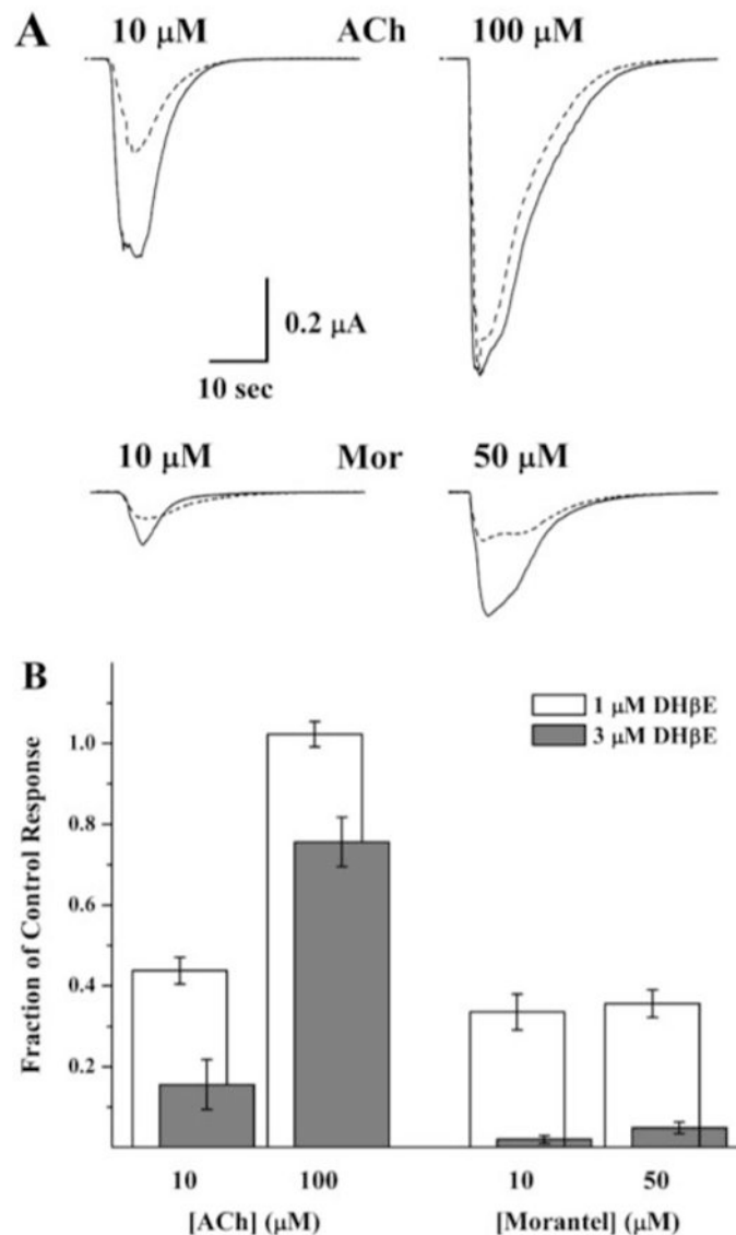
Fig. 5. DH \beta E inhibits morantel-evoked currents noncompetitively. A, currents, all from the same \alpha 3\beta 2 -expressing oocyte, evoked by ACh or morantel (solid traces) are overlaid with their pairs, the currents evoked by coapplication of the same concentration and 1.0 \mu\text{M} dihydro- \beta -erythroidine (DH \beta E; dashed traces). All applications were 5 s. B, collated data of the type shown in A are plotted to indicate the degree of inhibition by DH \beta E [i.e., the fraction of control current remaining upon coapplication with DH \beta E ( I_{+\text{DH}\beta\text{E}}/I_{\text{agonist alone}} )]. The open bars are inhibition by 1.0 \mu\text{M} DH \beta E ( n = 5 , one donor) and the solid bars are inhibition by 3.0 \mu\text{M} DH \beta E ( n = 8 , one donor, different from the 1 \mu\text{M} experiment). For both experiments, all 8 challenges were given to the entire set of oocytes. The choices of 10 and 50 \mu\text{M} morantel were constrained by the need to have measurable responses both in the absence and presence of DH \beta E and to avoid the self-inhibition at concentrations >50 \mu\text{M} (see Figure 2A). This 5-fold range constitutes the same relative change in evoked response as the 10-fold range for ACh.
