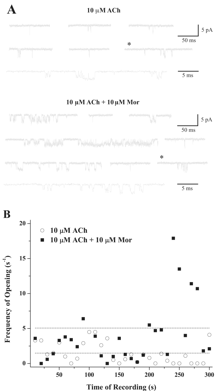
Fig. 3. Morantel increases the frequency of single-channel openings. A, representative single-channel current traces are shown from an experiment using 10 \mu M ACh alone (top) and with 10 \mu M morantel added (bottom) to the same outside-out patch held at -60 mV. Traces are not continuous; filtering was at 5 kHz. Downward deflections are the brief openings. The trace marked with * in each set is shown at the higher time resolution as the bottom trace in each set. B, the frequency of channel openings, calculated as averages in 10-s bins to approximate an “instantaneous” measure, is plotted for each entire 300-s recording for the experiment shown in A. The dashed lines indicate the overall average frequencies of 1.5 s^{-1} for ACh alone and 5.1 s^{-1} in the presence of morantel.
