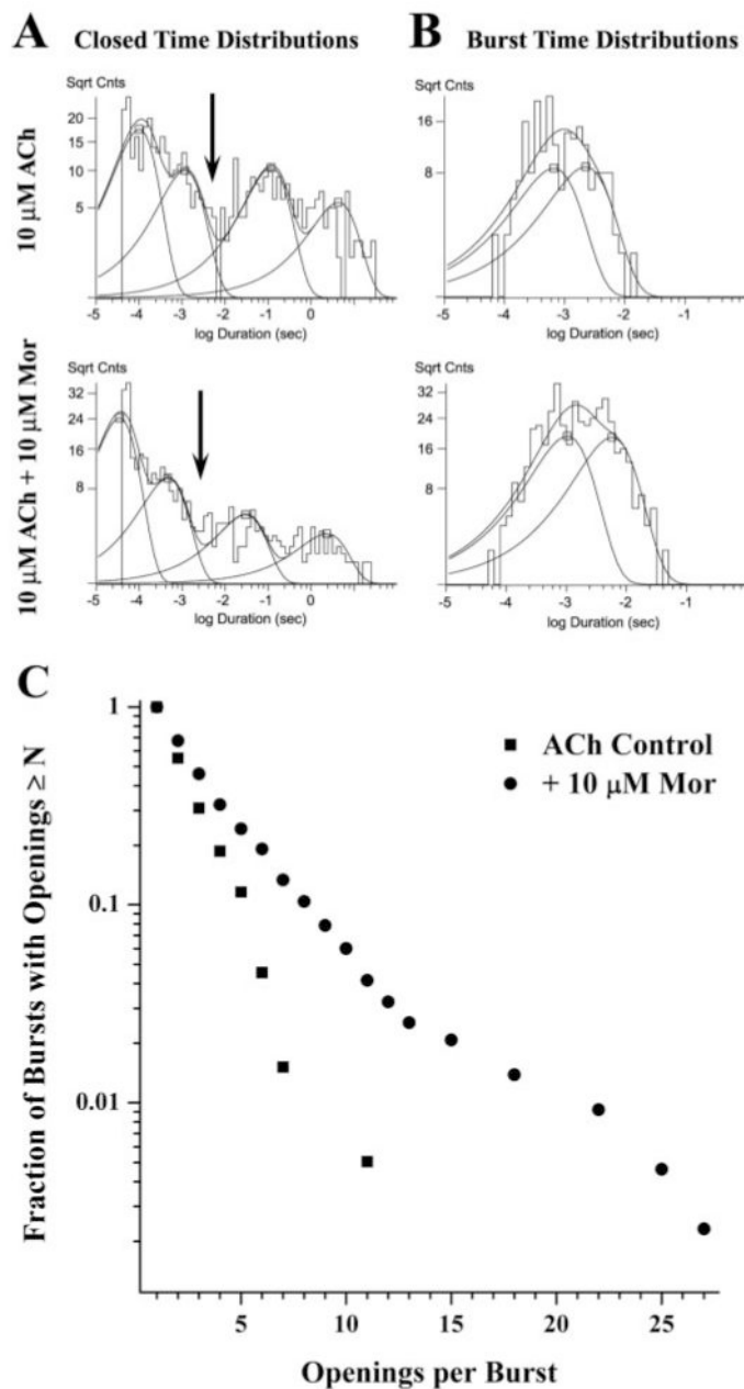
Fig. 4. Morantel increases the bursting behavior of single-channel openings. A, the closed time histograms for the experiment shown in Fig. 3 are given for ACh alone (top) and with morantel (bottom). The four-component fits were as follows (relative area, \tau in ms), for 10 \mu\text{M} ACh alone: 0.385, 0.112; 0.234, 1.12; 0.247, 110; 0.135, 4230; and with 10 \mu\text{M} Mor: 0.543, 0.052; 0.248, 0.664; 0.128, 47.6; 0.08, 1610. B, the burst time histograms for this same patch are given for ACh alone (top) and with morantel (bottom). The two-component fits were as follows (relative area, \tau in ms), for 10 \mu\text{M} ACh alone: 0.48, 0.669; 0.52, 2.17; and with 10 \mu\text{M} Mor: 0.57, 1.23; 0.43, 6.37. The arrows in A indicate t_{\text{critical}} = 3.0 ms, defining the burst (see Materials and Methods ). The ordinate in A and B is the square root of counts per bin. C, the distributions of the number of openings per burst for the two conditions in the experiment are plotted to indicate the difference in bursting character.
