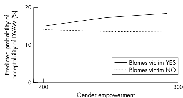
Figure 1 Graphical representation of significant interaction from three level multilevel analysis of the Eurobarometer 51.0, European Union.
