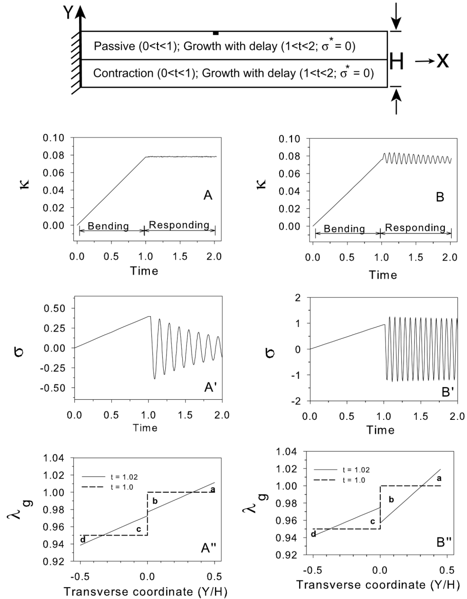
Figure 5. Cantilever beam oscillations. Bottom layer contracts for 0 \leq t \leq 1 (bending phase) and remains at maximum contraction thereafter; both layers grow in response to stress ( \sigma^* = 0 ) with a time delay for 1 < t \leq 2 (responding phase). (This model is the same as that of Fig. 4 except for the delayed response.) (A)–(A'') Materially homogeneous beam; stress oscillations occur without bending oscillations. (B)–(B'') Materially inhomogeneous beam (modulus of top layer > modulus of bottom layer); both stress and bending oscillations occur. (A,B) Beam curvature vs. time. (A',B') Bending stress vs. time at element indicated by filled rectangle in schematic. (A'',B'') Change in transverse distribution of \lambda_g during a small representative time interval (from t = 1.00 to t = 1.02 ). For the beam on the left, the increases and decreases in \lambda_g cancel out (area a = area d and area b = area c); hence the curvature does not oscillate. For the beam on the right, the transverse change in \lambda_g from t = 1.0 to t = 1.02 is not symmetric (B'': area a \neq area d and area b \neq area c), leading to bending oscillations. See text for details. Please see Fig. 3A for section used in A'',B''.
