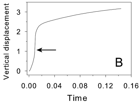
Figure 7. Elastic snap-through during invagination in a spherical shell (no fluid). (A) Undeformed (dotted) and deformed (solid) configurations. Shaded region denotes active region ( \sigma^* = 25.0 ; active modulus = 10 \times passive modulus); region immediately above the active region is passive; growth with \sigma^* = 0 everywhere else. Target stresses are specified in both the meridional and circumferential directions. Insert shows the configurations immediately before ( t = 0.009 ) and after ( t = 0.01 ) snap through. (B) Vertical displacement vs. time at node T (indicated in A). (C) Vertical displacement vs. \lambda_g at node T (indicated in A). Arrows in (B) and (C) denote the sudden increase in displacement due to snap through.
