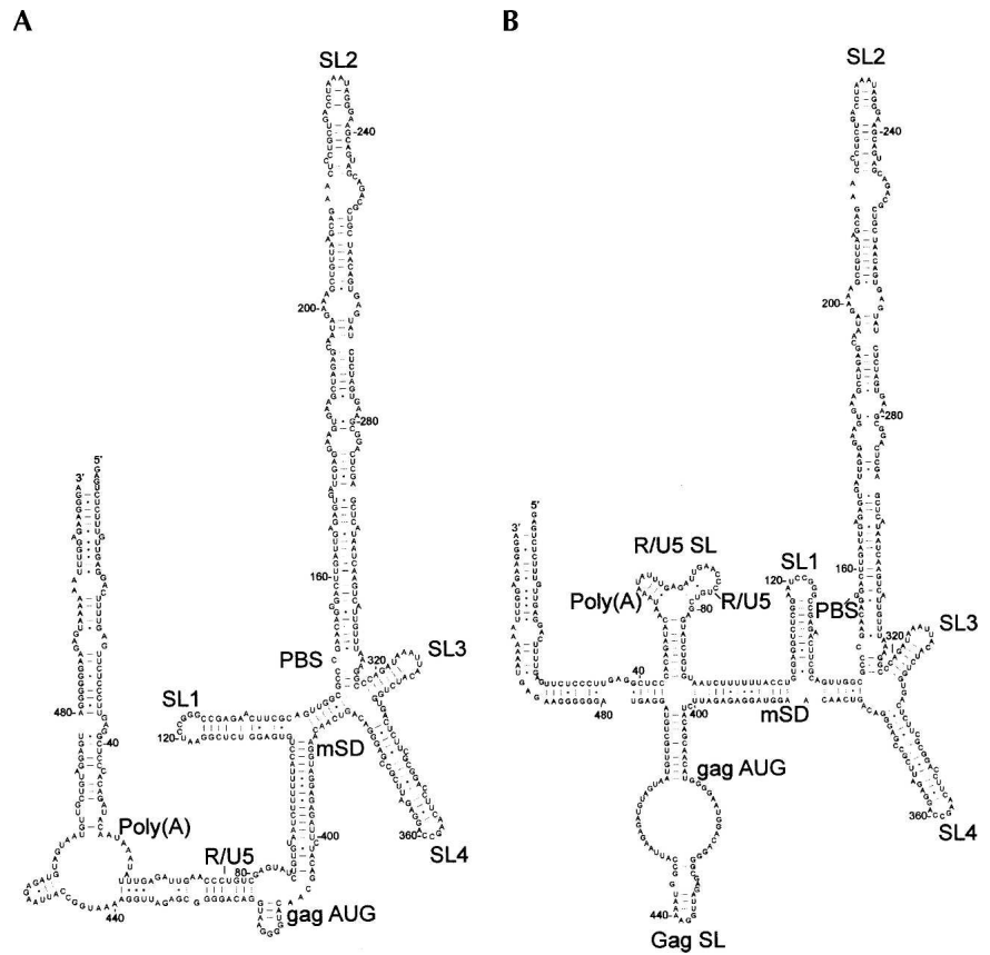
FIGURE 1. Minimal free-energy models of the FIV packaging signal RNA. Models were generated by the Mfold server using FIV Petaluma sequence RNA nt 1–511. The two most stable structures are shown. (A) \delta G = -180.83 kcal/mol; (B) \delta G = -181.60 kcal/mol.
