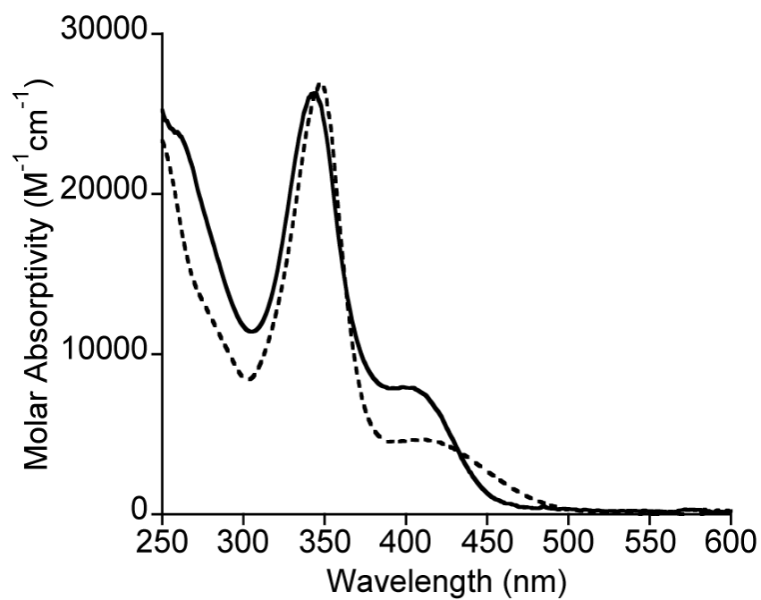
Figure 1. UV-vis spectra of L^{\text{Me}_2}\text{Cu-Ge}[(\text{NMes})_2(\text{CH})_2] ( 1a , solid line) and L^{\text{Me}_2}\text{Cu-Ge}[\text{N}(\text{SiMe}_3)_2]_2 ( 1b , dashed line) in THF at 25 °C.
