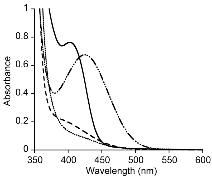
Figure 4. UV-vis spectra of L^{\text{Me}_2}\text{Cu-Ge}[(\text{NMes})_2(\text{CH})_2] ( 1a ) in THF (0.1 mM) at -80\text{ }^\circ\text{C} (solid line), the immediate product of oxygenation ( intermediate A , Scheme 4, dotted line), the species resulting after allowing intermediate A to stand for 10 minutes ( intermediate B , dashed line), and the product resulting from warming of intermediate B to -65\text{ }^\circ\text{C} (dot-dash line).
