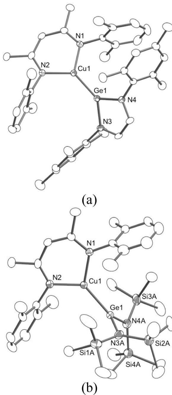
Figure 2. Molecular structures of (a) 1a and (b) 1b with heteroatoms labeled, all atoms as 50% thermal ellipsoids, and hydrogen atoms omitted for clarity. Selected bond distances (Å) and angles (deg): (a) Cu1-N1, 1.9194(17); Cu1-N2, 1.9153(17); Cu1-Ge1, 2.2138(4); N1-Cu1-N2/N3-Ge1-N4, 44.03(7). (b) Cu1-N1, 1.956(3); Cu1-N2, 1.938(3); Cu1-Ge1, 2.2492(4); N1-Cu1-N2/N3A-Ge1-N4A, 88.15(21). For 1b , only one conformation of the disordered N(SiMe 3 ) 2 groups is shown.
