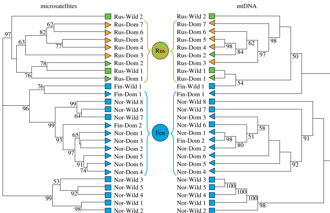
Figure 2. Population dendrograms as inferred from microsatellite and mtDNA data. Wild and domestic populations are represented by squares and triangles, respectively. Geographical origins are represented by different colours. Blue, Fennoscandia; Orange, western Russia; Green, eastern Russia. Two putative origins for domestication (Russia and Fennoscandia) are indicated by filled circles between the trees.
