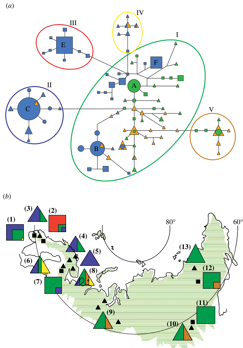
Figure 1. (a) Median-joining network for mitochondrial DNA haplotypes found in Eurasian reindeer. Haplotypes found only in wild herds are represented by squares, whereas the triangles represent domestic haplotypes. Circles represent haplotypes found in both wild and domestic herds. Blue haplotypes are found in Fennoscandia, whereas the orange and green haplotypes represent western and eastern Russia, respectively. Five different haplotype clusters (haplogroups, I–V) are encircled with different colours. Haplotypes that are directly mentioned in the text are labelled with capital letters. (b) Haplogroup frequencies in wild (squares) and domestic (triangles) reindeer herds. Populations are pooled according to geography and whether they are wild or domestic herds: (1) southwestern Norway wild (Nor-Wild 6–8), (2) central Norway wild (Nor-Wild 1–5), (3) central Norway domestic (Nor-Dom 1–3), (4) northern Norway domestic (Nor-Dom 4–6), (5) northern Finland domestic (Fin-Dom 2), (6) eastern Finland domestic (Fin-Dom 1), (7) eastern Finland wild (Fin-Wild 1), (8) northwestern Russia domestic (Rus-Dom 6 and 7), (9) north-central Russia domestic (Rus-Dom 3–5), (10) southeastern Russia domestic (Rus-Dom 2), (11) southeastern Russia wild (Rus-Wild 2), (12) northeastern Russia wild (Rus-Wild 1), (13) northeastern Russia domestic (Rus-Dom 1; see table S1 in the electronic supplementary material). Colours representing the different haplogroups are the same that are used to mark them in (a). Green lines in the map indicate the distribution range of Eurasian reindeer.
