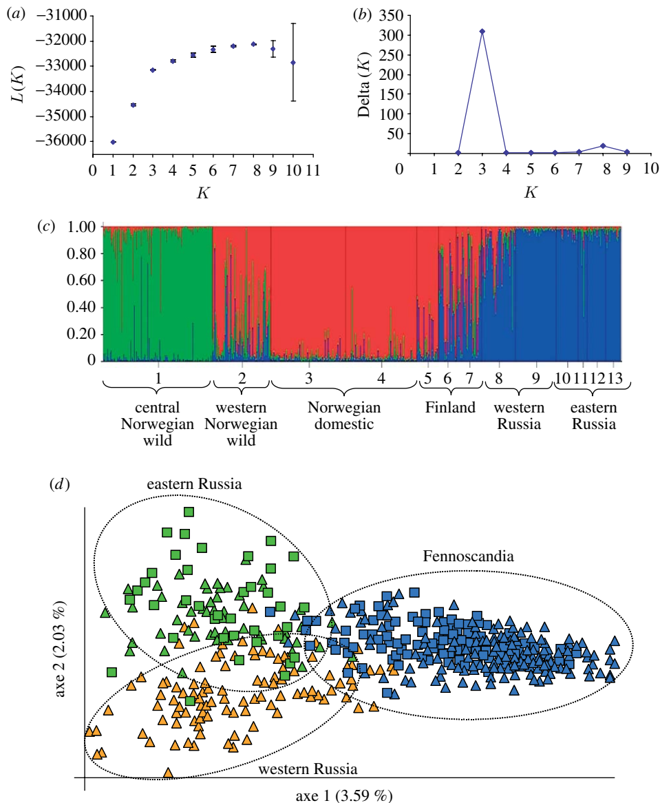
Figure 3. Clustering analysis in Eurasian reindeer herds, using (a–c) Bayesian assignment and (d) a factorial correspondence analysis. (a) Mean likelihood ( L(K) ( \pm s.d.)) over 10 runs dividing the entire dataset into K populations, for K values between 1 and 10. (b) Delta ( K ) where the modal value of the distribution is considered as the highest level of structuring, in our case three clusters. (c) Individual assignment to each of the three clusters, where the numbers refer to the same populations as given in figure legend 1b. Each individual is represented by a line and the proportion of each colour indicates proportion of ancestry from each group. (d) Factorial correspondence analysis of Eurasian reindeer, after excluding wild reindeer from central Norway. The graphics shows the two first axes. Wild and domestic individuals are symbolized by squares and triangles, respectively, and the colours are the same as given in figure legend 2.
