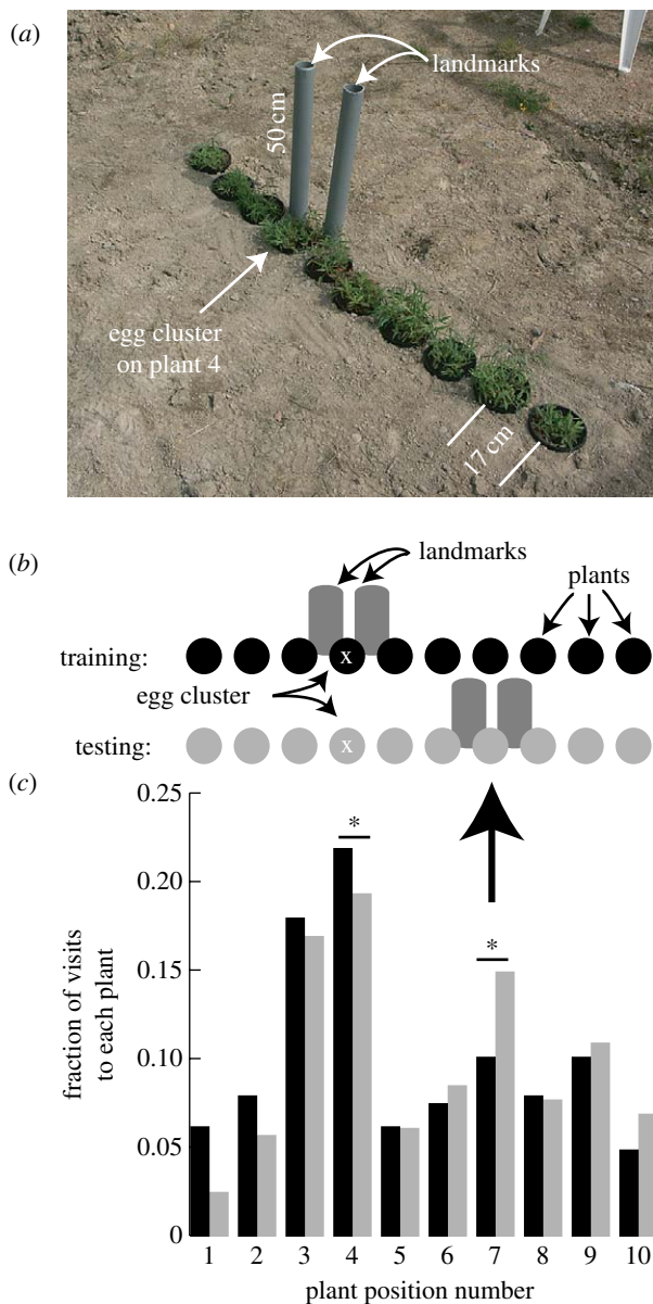
Figure 5. The egg-flanked landmark experiment. (a) An array of V. spicata plants during the training portion of the experiment. The two grey cylinders (landmarks) are shifted between the wasp training and testing periods. (b) Schematic of the experiment. Filled circles, plants during training (black) and testing (grey); White X, the plant with host eggs on it; grey bars, the landmarks. The thick arrow points to the plant expected to receive increased visitation during testing. (c) The fraction of visits to each plant by H. horticola during training (black bars) and testing (grey bars). The asterisk indicates a significant difference between the number of visits between the last day of training and the first day of testing. Altogether, there were 1060 observed visits to plants.
