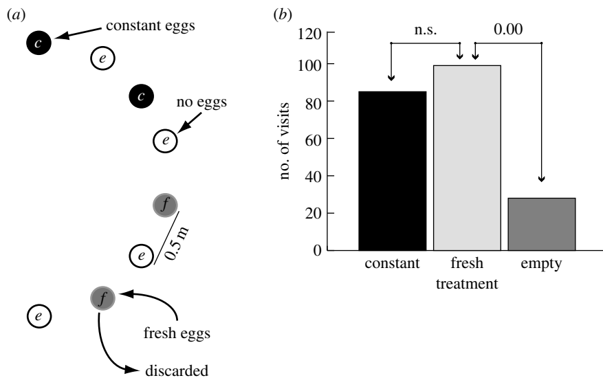
Figure 3. (a) The arrangement of potted P. lanceolata plants in the field rate of visitation experiment. The constant (c) plants with host egg clusters on them that were left in place throughout the experiment; the (f), fresh plants with host eggs on them that were replaced each day if visited by wasps; the empty (e), plants without host eggs. Two arrays 10 m apart were observed simultaneously. (b) The number of visits by H. horticola to plants in each of the three treatments described above. The numbers above the bars represent the p values of post hoc comparisons among treatments.
