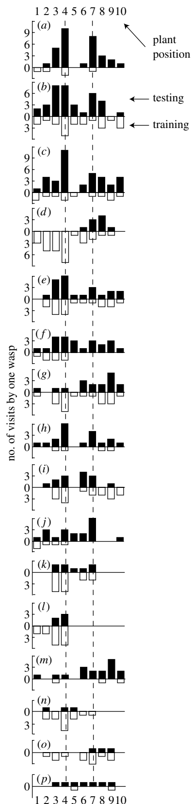
Figure 6. The number of visits to each plant by 16 H. horticola in one replicate of the egg-flanked landmark experiment. Each bar plot (a–p) shows visitation by a single wasp. Inverted white bars, visits during training; black bars, visits during testing. The wasps shown are those that visited the array at least twice during both training and testing. Dashed lines, plant 4 (with the eggs and landmarks during training) and plant 7 (which received the landmarks during testing). Of these 16 wasps, 13 increased their visits to plant 7 when the landmarks were moved.
