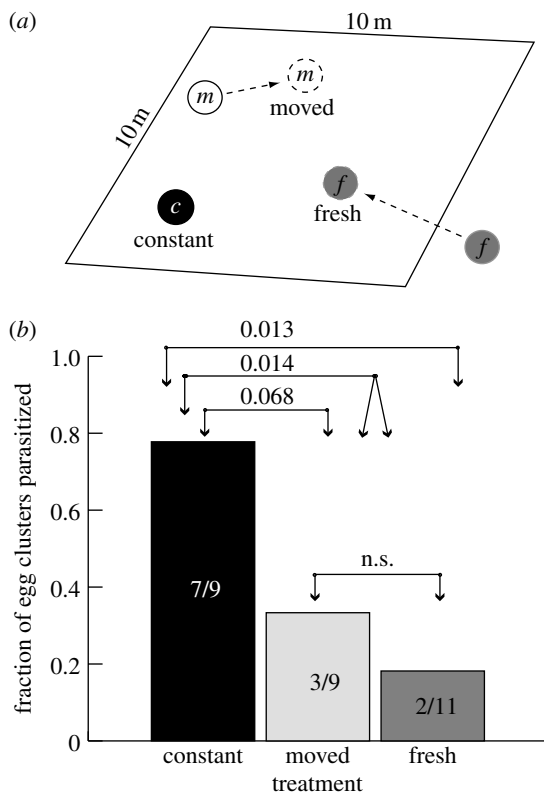
Figure 2. (a) Schematic of constant ( c ), moved ( m ) and fresh ( f ) egg clusters in one replicate in one plot of the field experiment on rate of parasitism. There are three plots in the experiment with four replicates of each treatment in each plot. (b) The fraction of egg clusters parasitized by H. horticola in each of the three treatments. The numbers above the bars are the p values of post hoc comparisons among treatments.
