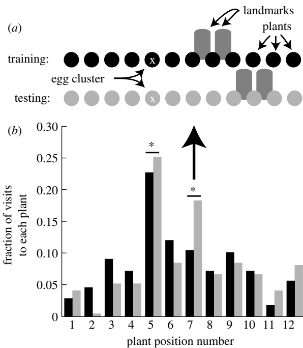
Figure 7. The plant-flanked landmark experiment. The symbols and shades are as shown in figure 5. (a) Schematic of the experiment. (b) The fraction of visits to each plant by H. horticolae during training and testing. The asterisk indicates a statistically significant difference between the number of visits between the last day of training and the first day of testing. Altogether, there were 1442 visits to plants.
