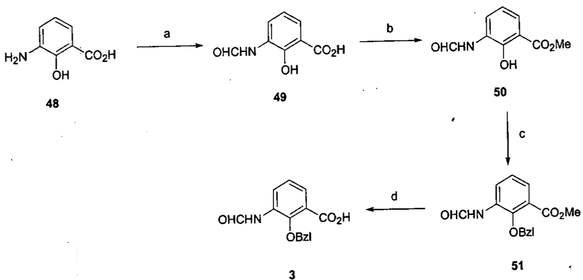
Scheme 7.
