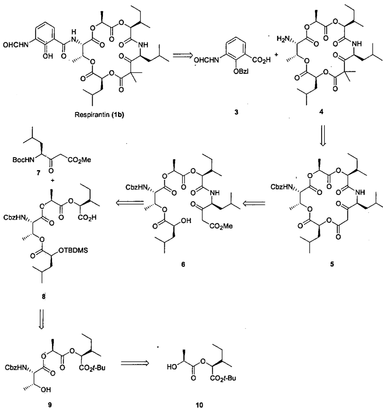
Scheme 1. Retrosynthetic Analysis of Respirantin
