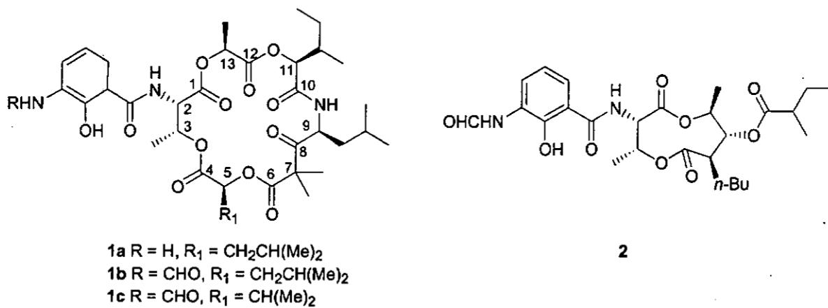
Figure 1. Kitastatin, respirantin and valeryl modification. (+)-Antimycin A 3b .
