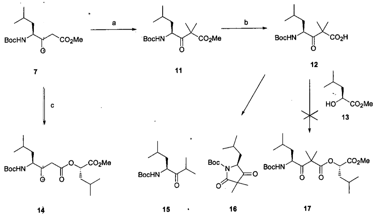
Scheme 2.
