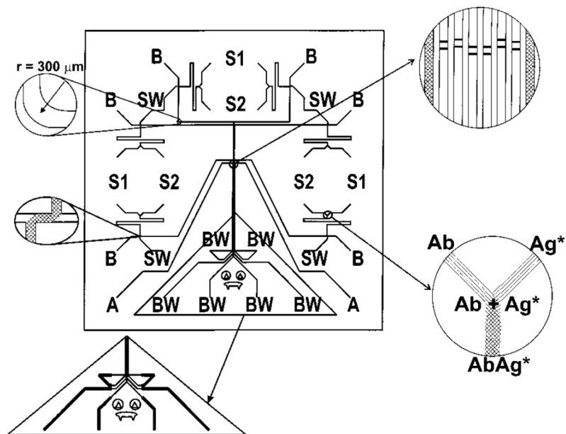
Figure 3. Illustration of a microchip design for six simultaneous CE-based immunoassays. Each channel manifold is capable of online mixing of immunoassay reagents (from reservoirs S1 and S2) followed by injection onto capillary electrophoresis channels for separation and detection. [26]
