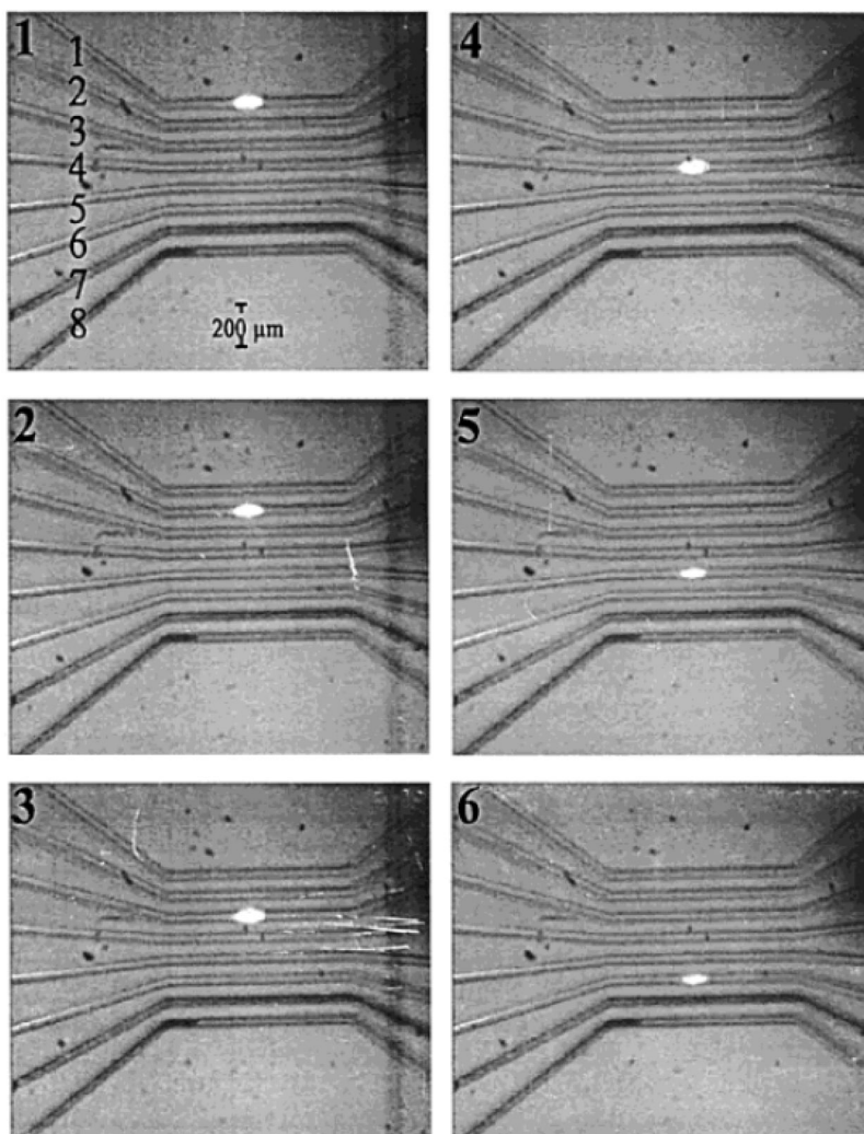
Figure 1. Six CCD images showing the positioning of a laser spot scanned across eight microfluidic channels using AOD. This type of laser scanning was used to monitor parallel separations on a microchip with a PMT detector. [27]
