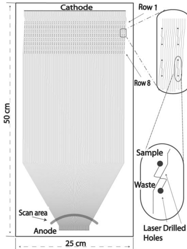
Figure 4. One of two microfabricated plates used in a 768-lane system for DNA sequencing. Each plate consists of 384 parallel channels. Separation and detection is performed on one plate while another is regenerated. Details on the automated instrumentation used are available here. [62]
