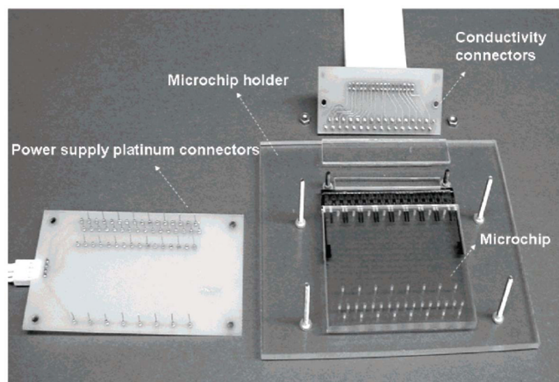
Figure 2. Illustration of a workstation consisting of a microfluidic chip, chip holder, and necessary electrical connection devices for parallel CE separations and electrochemical detection. The device, fabricated from polycarbonate, allowed 16 parallel separations of amino acids, peptides, proteins, and DNA fragments. [41]
