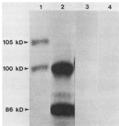
FIG. 1. Comparison of MSP-1 complexes between the Florida and Washington-O isolates of A. marginale . Organisms from each isolate were radiolabeled with [ 35 S]methionine, detergent disrupted, and immunoprecipitated with monoclonal antibody ANA 22B1, which recognizes a conserved MSP-1 epitope. Immunoprecipitates were identified by polyacrylamide gel electrophoresis with fluorography. Florida isolate proteins were immunoprecipitated with monoclonal antibody ANA 22B1 (lane 1) or control monoclonal antibody TRYP 1E1 (lane 3). Washington-O isolate proteins were immunoprecipitated with ANA 22B1 (lane 2) or TRYP 1E1 (lane 4). Arrows in the left margin designate the apparent molecular masses, in kilodaltons, of the polypeptides.
