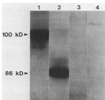
FIG. 2. Antigenic identity of MSP-1 polypeptides in the Washington-O isolate of A. marginale . Washington-O isolate antigens were separated by sodium dodecyl sulfate-polyacrylamide gel electrophoresis and transferred to nitrocellulose. Antibody binding was detected by reaction with 125 I-protein A, followed by autoradiography. Lanes: 1, rabbit antibody R911 (defined against the Florida isolate 100-kDa polypeptide); 2, monoclonal antibody ANA 22B1 (defined against the Florida isolate 105-kDa polypeptide); 3, control rabbit antibody (against E. coli ); 4, control monoclonal antibody TRYP 1E1.
