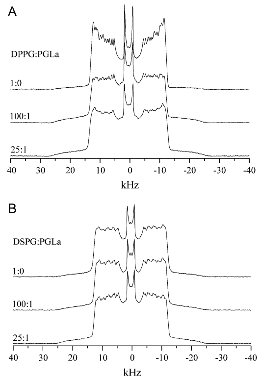
FIGURE 3 ^2\text{H} -NMR fluid-phase spectra of chain-deuterated DPPG vesicles at 45°C (A) and DSPG at 60°C (B), containing PGLa at different lipid/peptide ratios.
