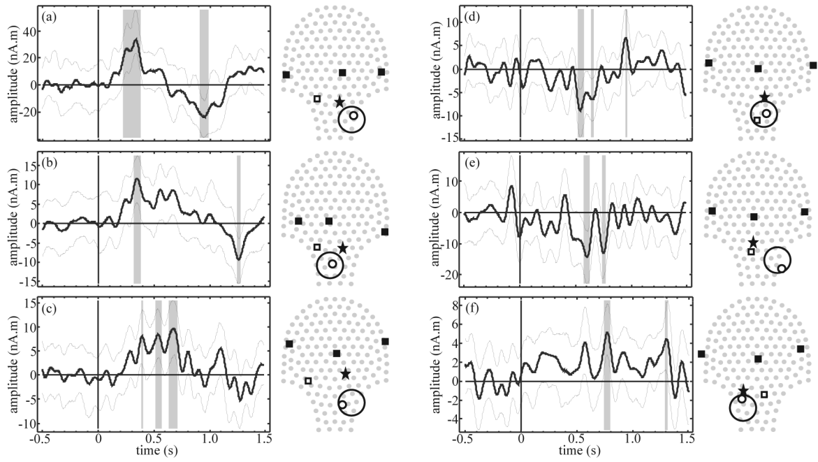
Figure 5. Model search results from fetal response to flash stimulation for each of the best 3 SNR datasets (a – c) and poorest 3 SNR datasets (d – f). For each example, left: time course of the one best source (thick line) with 95% confidence interval (thin lines) and statistically significant time segments (gray bands); right: projection of sensor array (gray dots) superimposed with localization coil positions (filled squares), 4 th coil position (open square), estimated fetal heart location (star), and best source location (small circle) with head model (large circle).
