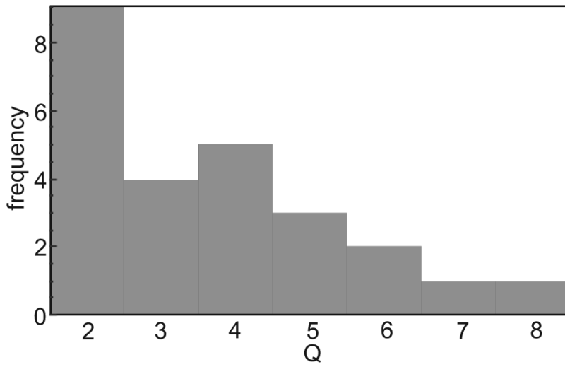
Figure 4. Histogram of Q for 25 datasets
