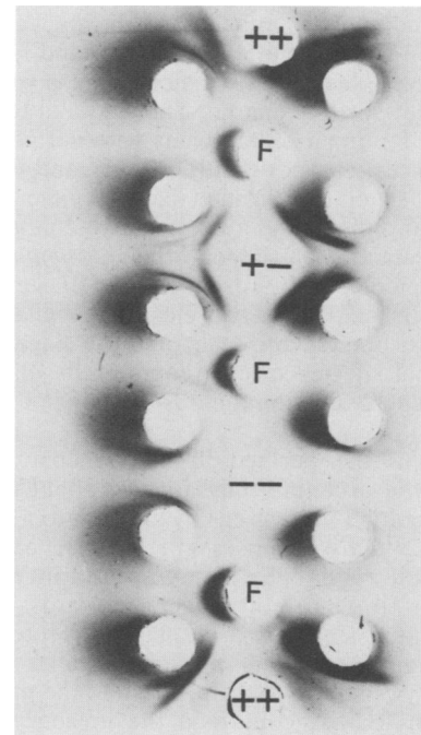
FIG. 8. Counterimmunoelectrophoresis of sheared F^+M^+ flagella (F), or acid-extracted material from F^+M^+ (++) and F^+M^- (+-) C. jejuni strains with F^+M^+ -immune rabbit serum. The antigen-containing wells are in the center with the F^+M^+ antibody-containing wells on the sides. The anode is on the right, and the cathode is on the left.
