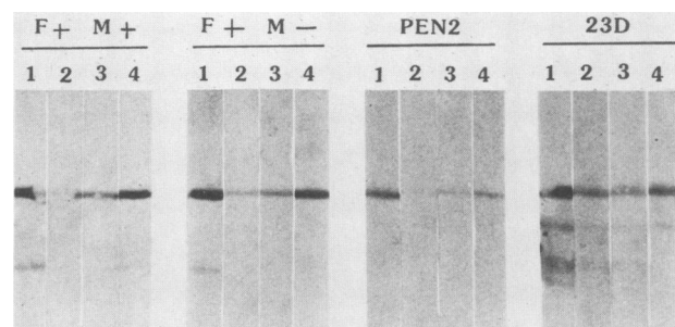
FIG. 6. Western blots of purified Campylobacter flagella with unabsorbed and absorbed homologous antisera. Flagellar preparations are from (left to right) F^+M^+ , F^+M^- , PEN 2 C. jejuni strains, and 23D C. fetus strain. For each preparation, lane 1 represents the unabsorbed antiserum raised to whole homologous cells, whereas lanes 2 through 4 represent that antiserum absorbed with various cells. Absorptions of the antisera to F^+M^+ , F^+M^- , and 23D are with F^+M^+ (lanes 2), F^-M^- cells (lanes 3), and PEN 2 cells (lanes 4). Absorptions of PEN 2 antiserum are with PEN 2 cells (lane 2), F^+M^+ cells (lane 3), and F^-M^- cells (lane 4).
