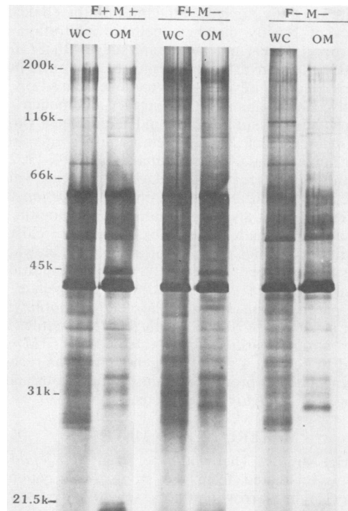
FIG. 1. SDS-PAGE (10% acrylamide) profile of whole cell (WC) and outer membrane (OM) by sarcosyl extraction of the three related C. jejuni strains. Molecular weights of marker proteins are indicated at left. The F - M - strain does not include the major band seen in the 63 kDa region present in similar preparations of the other two strains.
