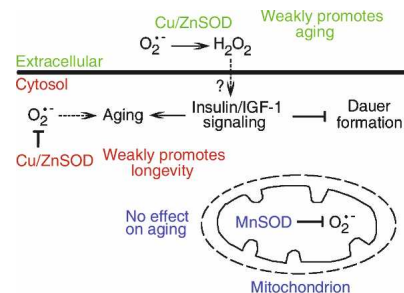
Figure 4. Influence of SOD and O_2^- on aging. This scheme shows a synthesis of conclusions drawn from the present study. Different SOD isoforms (and by deduction, the corresponding O_2^- pools) have different effects on aging. Extracellular Cu/ZnSOD weakly inhibits dauer formation and promotes aging, potentially by generating H_2O_2 , which crosses into the cell and stimulates insulin/IGF-1 signaling by inhibiting redox-sensitive phosphatases. Cytosolic Cu/ZnSOD weakly promotes longevity, perhaps by protecting against molecular damage ( sod-1 does not influence daf-2 Daf-c). Mitochondrial MnSOD has no detectable effect on aging. Arrow with dotted line implies a weak effect.
